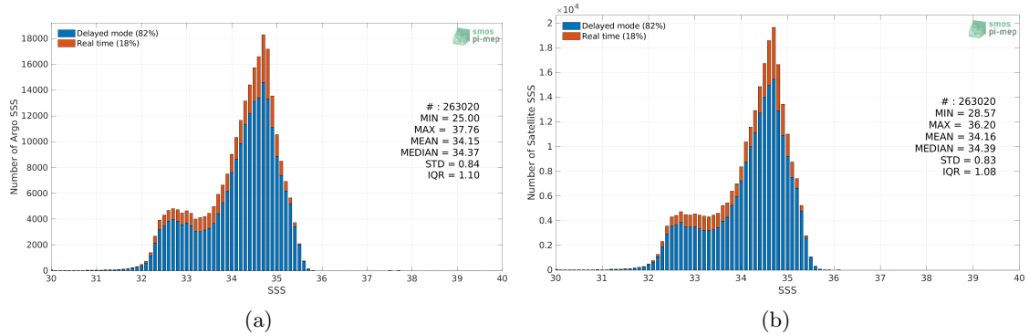
Figure 2: Histograms of SSS from Argo (a) and CCI SSS L4 Merged-OI v3.2 - 30-day running (ESA) (b) considering all match-up pairs per bins of 0.1 over the North Pacific Ocean Pi-MEP region and for the full satellite product period.
