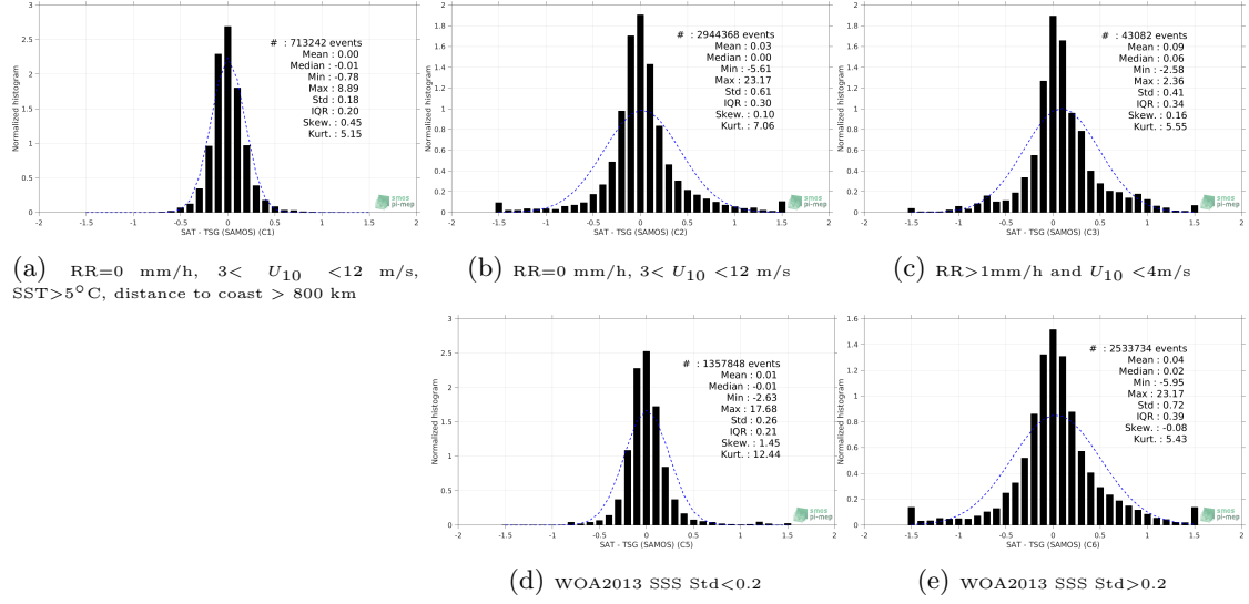
Figure 13: Normalized histogram of \Delta\text{SSS} (CCI SSS L4 Merged-OI v2.31 - 30-day running (ESA) - TSG (SAMOS)) for 5 different subdatasets corresponding to: RR=0 mm/h, 3 < U_{10} < 12 m/s, SST>5°C, distance to coast > 800 km (a), RR=0 mm/h, 3 < U_{10} < 12 m/s (b), RR>1mm/h and U_{10} < 4 m/s (c), WOA2013 SSS Std<0.2 (d), WOA2013 SSS Std>0.2 (e).
