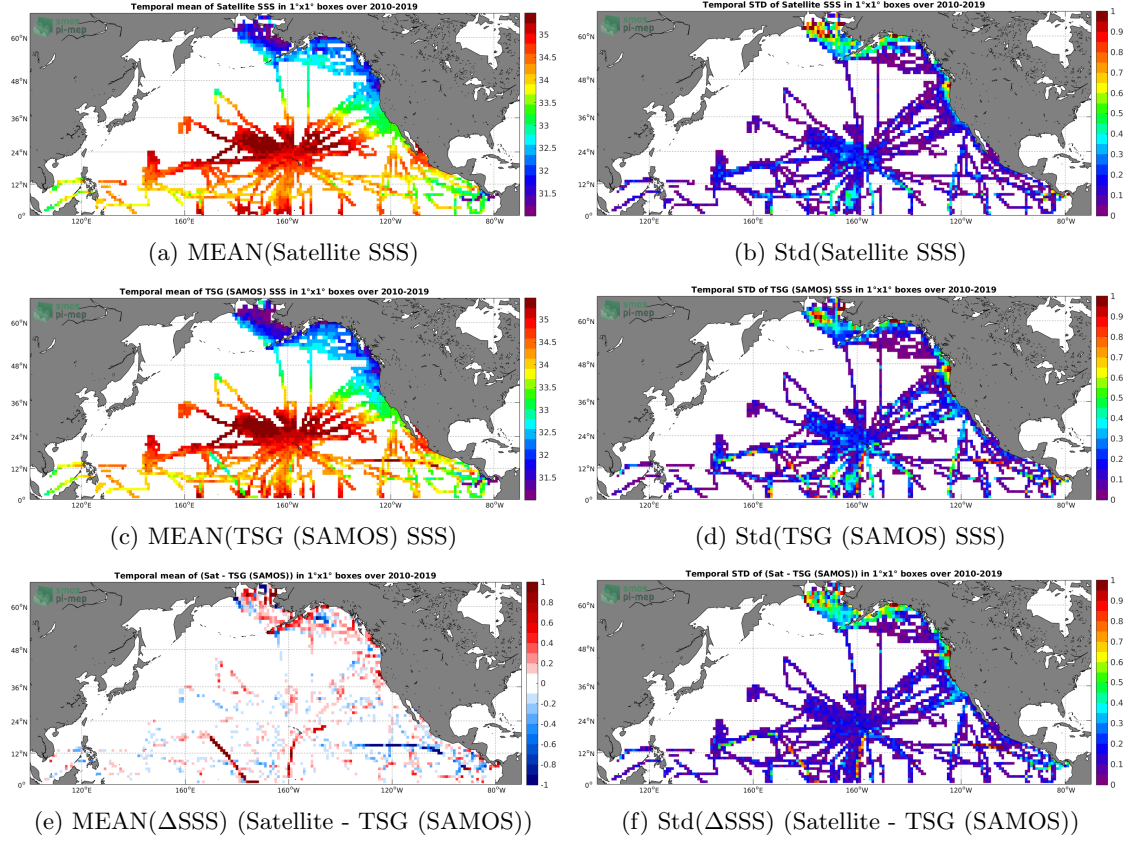
Figure 6: Temporal mean (left) and Std (right) of SSS from CCI SSS L4 Merged-OI v2.31 - 30-day running (ESA) (top), TSG (SAMOS) (middle), and of \Delta SSS (Satellite - TSG (SAMOS)). Only match-up pairs are used to generate these maps.
