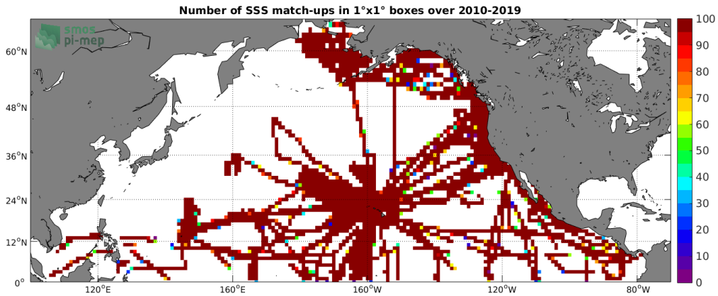
Figure 4: Number of SSS match-ups between TSG (SAMOS) SSS and the CCI SSS L4 Merged-OI v2.31 - 30-day running (ESA) SSS product for the North Pacific Ocean Pi-MEP region over 1^\circ \times 1^\circ boxes and for the full satellite product period.
