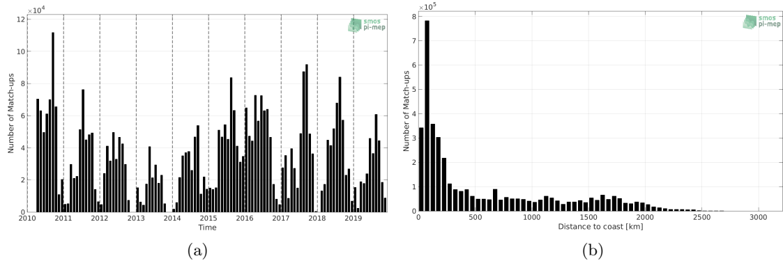
Figure 1: Number of match-ups between TSG (SAMOS) and CCI SSS L4 Merged-OI v2.31 - 30-day running (ESA) SSS as a function of time (a) and as function of the distance to coast (b) over the North Pacific Ocean Pi-MEP region and for the full satellite product period.
