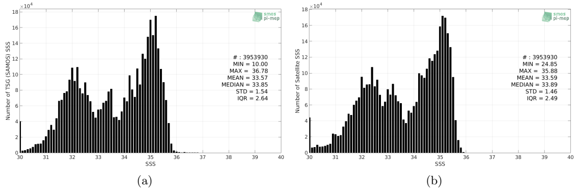
Figure 2: Histograms of SSS from TSG (SAMOS) (a) and CCI SSS L4 Merged-OI v2.31 - 30-day running (ESA) (b) considering all match-up pairs per bins of 0.1 over the North Pacific Ocean Pi-MEP region and for the full satellite product period.
