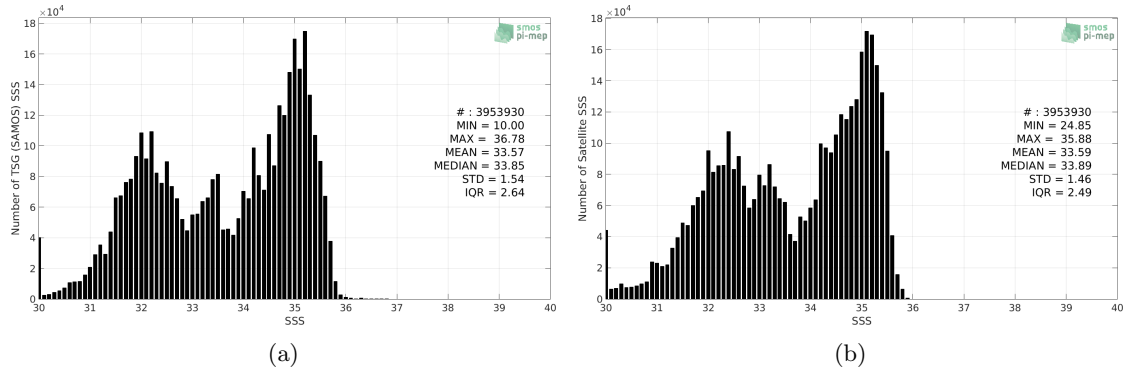
Figure 2: Histograms of SSS from TSG (SAMOS) (a) and CCI L4 Merged-OI v2.31 - 30-day running (ESA) (b) considering all match-up pairs per bins of 0.1 over the North Pacific Ocean Pi-MEP region and for the full satellite product period.
