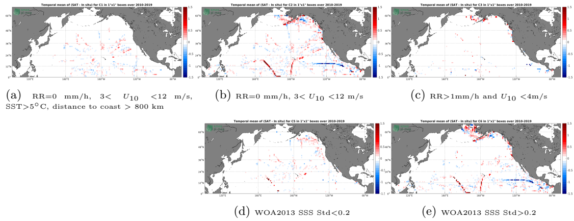
Figure 12: Temporal mean gridded over spatial boxes of size 1^\circ \times 1^\circ of \Delta SSS (CCI L4 Merged-OI v2.31 - 30-day running (ESA) - TSG (SAMOS)) for 5 different subdatasets corresponding to: RR=0 mm/h, 3 < U_{10} < 12 m/s, SST > 5^\circ C , distance to coast > 800 km (a), RR=0 mm/h, 3 < U_{10} < 12 m/s (b), RR > 1 mm/h and U_{10} < 4 m/s (c), WOA2013 SSS Std < 0.2 (d), WOA2013 SSS Std > 0.2 (e).
