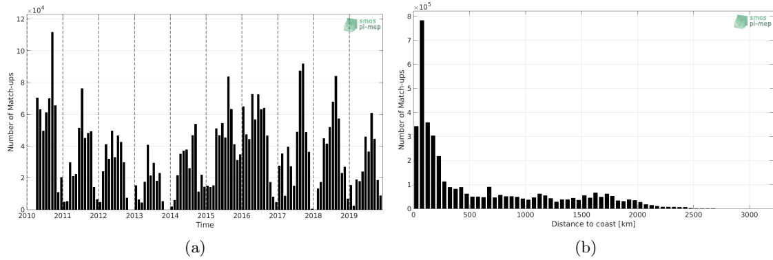
Figure 1: Number of match-ups between TSG (SAMOS) and CCI L4 Merged-OI v2.31 - 30-day running (ESA) SSS as a function of time (a) and as function of the distance to coast (b) over the North Pacific Ocean Pi-MEP region and for the full satellite product period.
