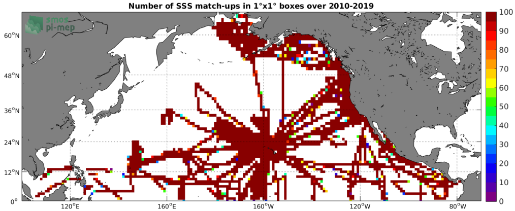
Figure 4: Number of SSS match-ups between TSG (SAMOS) SSS and the CCI L4 Merged-OI v2.31 - 30-day running (ESA) SSS product for the North Pacific Ocean Pi-MEP region over 1^\circ \times 1^\circ boxes and for the full satellite product period.
