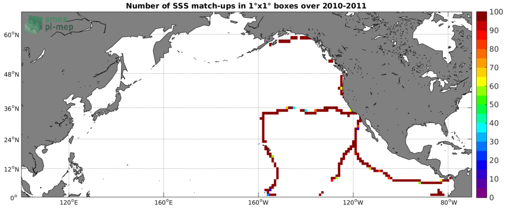
Figure 4: Number of SSS match-ups between TSG (GOSUD-Sailing-ship) SSS and the CCI SSS L4 Merged-OI v2.31 - 30-day running (ESA) SSS product for the North Pacific Ocean Pi-MEP region over 1^\circ \times 1^\circ boxes and for the full satellite product period.
