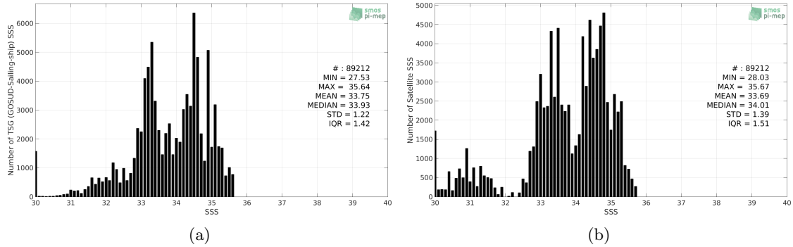
Figure 2: Histograms of SSS from TSG (GOSUD-Sailing-ship) (a) and CCI SSS L4 Merged-OI v2.31 - 30-day running (ESA) (b) considering all match-up pairs per bins of 0.1 over the North Pacific Ocean Pi-MEP region and for the full satellite product period.
