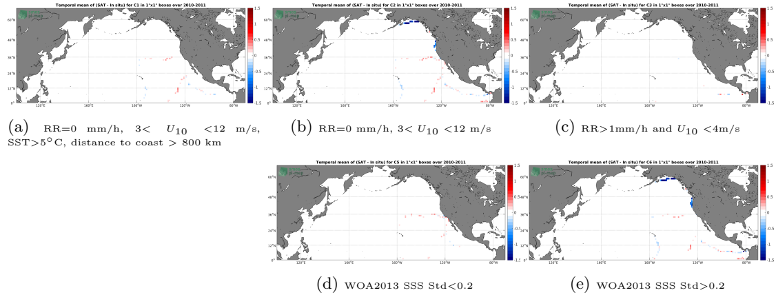
Figure 12: Temporal mean gridded over spatial boxes of size 1^\circ \times 1^\circ of \Delta SSS (CCI SSS L4 Merged-OI v2.31 - 30-day running (ESA) - TSG (GOSUD-Sailing-ship)) for 5 different subdatasets corresponding to: RR=0 mm/h, 3 < U_{10} < 12 m/s, SST >5^\circ\text{C} , distance to coast > 800 km (a), RR=0 mm/h, 3 < U_{10} < 12 m/s (b), RR >1 mm/h and U_{10} < 4 m/s (c), WOA2013 SSS Std <0.2 (d), WOA2013 SSS Std >0.2 (e).
