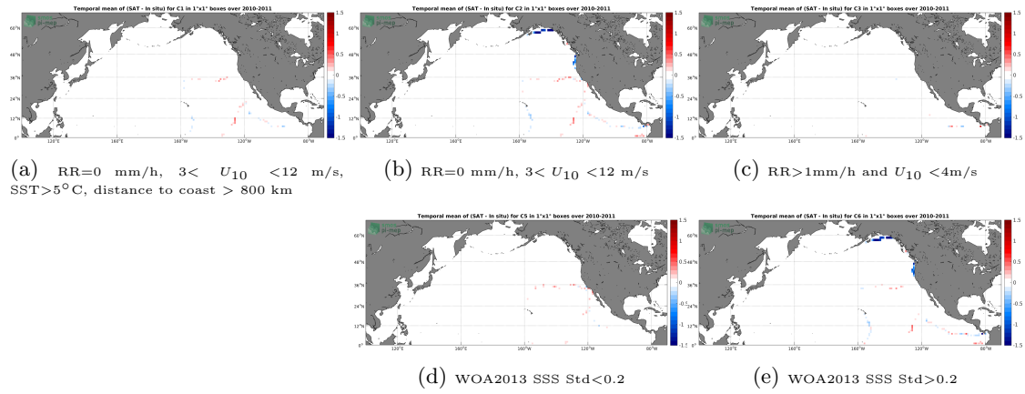
Figure 12: Temporal mean gridded over spatial boxes of size 1^\circ \times 1^\circ of \Delta SSS (CCI L4 Merged-OI v2.31 - 30-day running (ESA) - TSG (GOSUD-Sailing-ship)) for 5 different subdatasets corresponding to: RR=0 mm/h, 3 < U_{10} < 12 m/s, SST >5^\circ\text{C} , distance to coast > 800 km (a), RR=0 mm/h, 3 < U_{10} < 12 m/s (b), RR >1 mm/h and U_{10} < 4 m/s (c), WOA2013 SSS Std <0.2 (d), WOA2013 SSS Std >0.2 (e).
