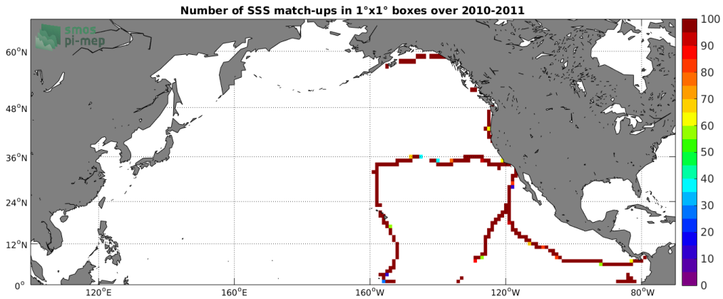
Figure 4: Number of SSS match-ups between TSG (GOSUD-Sailing-ship) SSS and the CCI L4 Merged-OI v2.31 - 30-day running (ESA) SSS product for the North Pacific Ocean Pi-MEP region over 1°x1° boxes and for the full satellite product period.
