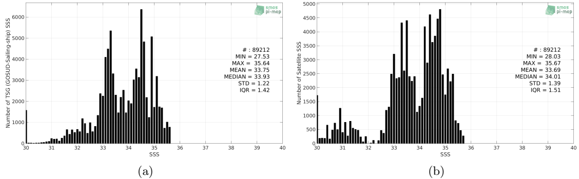
Figure 2: Histograms of SSS from TSG (GOSUD-Sailing-ship) (a) and CCI L4 Merged-OI v2.31 - 30-day running (ESA) (b) considering all match-up pairs per bins of 0.1 over the North Pacific Ocean Pi-MEP region and for the full satellite product period.
