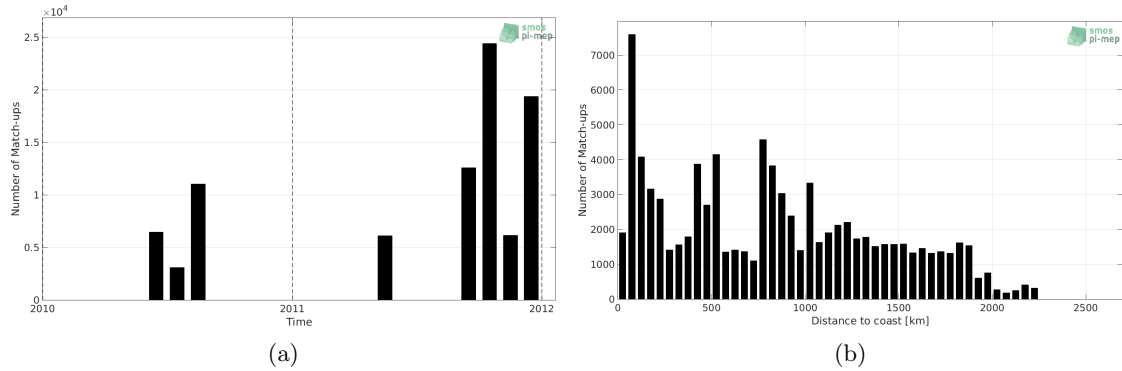
Figure 1: Number of match-ups between TSG (GOSUD-Sailing-ship) and CCI L4 Merged-OI v2.31 - 30-day running (ESA) SSS as a function of time (a) and as function of the distance to coast (b) over the North Pacific Ocean Pi-MEP region and for the full satellite product period.
