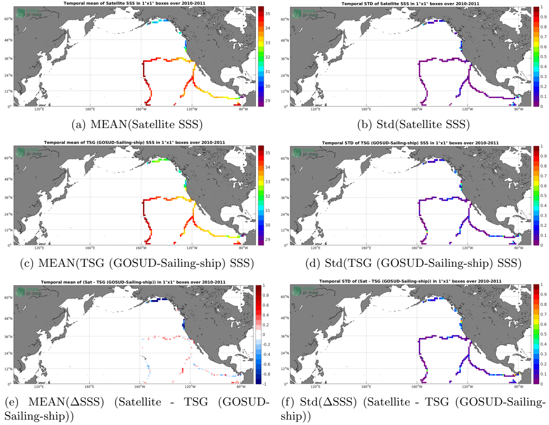
Figure 6: Temporal mean (left) and Std (right) of SSS from CCI L4 Merged-OI v2.31 - 30-day running (ESA) (top), TSG (GOSUD-Sailing-ship) (middle), and of \Delta SSS (Satellite - TSG (GOSUD-Sailing-ship)). Only match-up pairs are used to generate these maps.
