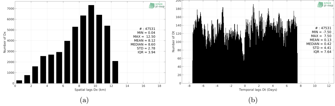
Figure 5: Histograms of the spatial (a) and temporal (b) lags between the time of the TSG (GOSUD-Research-vessel) measurements and the date of the corresponding CCI SSS L4 Merged-OI v2.31 - 30-day running (ESA) SSS product.
