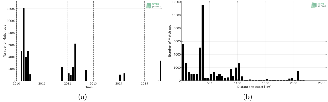
Figure 1: Number of match-ups between TSG (GOSUD-Research-vessel) and CCI SSS L4 Merged-OI v2.31 - 30-day running (ESA) SSS as a function of time (a) and as function of the distance to coast (b) over the North Pacific Ocean Pi-MEP region and for the full satellite product period.
