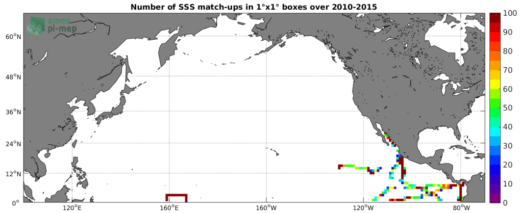
Figure 4: Number of SSS match-ups between TSG (GOSUD-Research-vessel) SSS and the CCI SSS L4 Merged-OI v2.31 - 30-day running (ESA) SSS product for the North Pacific Ocean Pi-MEP region over 1^\circ \times 1^\circ boxes and for the full satellite product period.
