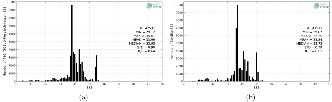
Figure 2: Histograms of SSS from TSG (GOSUD-Research-vessel) (a) and CCI SSS L4 Merged-OI v2.31 - 30-day running (ESA) (b) considering all match-up pairs per bins of 0.1 over the North Pacific Ocean Pi-MEP region and for the full satellite product period.
