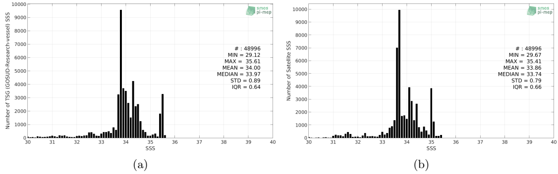
Figure 2: Histograms of SSS from TSG (GOSUD-Research-vessel) (a) and CCI L4 Merged-OI v2.31 - 30-day running (ESA) (b) considering all match-up pairs per bins of 0.1 over the North Pacific Ocean Pi-MEP region and for the full satellite product period.
