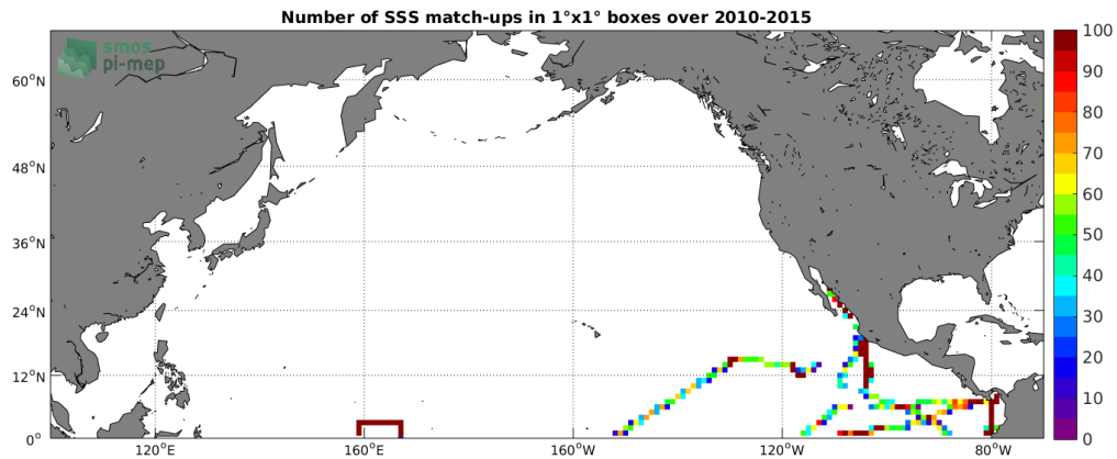
Figure 4: Number of SSS match-ups between TSG (GOSUD-Research-vessel) SSS and the CCI L4 Merged-OI v2.31 - 30-day running (ESA) SSS product for the North Pacific Ocean Pi-MEP region over 1^\circ \times 1^\circ boxes and for the full satellite product period.
