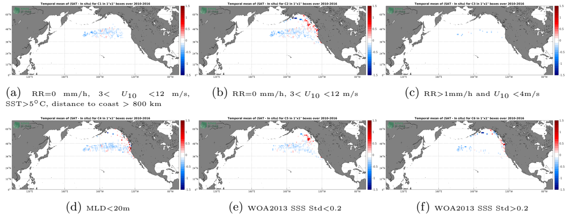
Figure 12: Temporal mean gridded over spatial boxes of size 1^\circ \times 1^\circ of \Delta SSS (CCI SSS L4 Merged-OI v2.31 - 30-day running (ESA) - Sea mammals) for 6 different subdatasets corresponding to: RR=0 mm/h, 3 < U_{10} < 12 m/s, SST >5^\circ\text{C} , distance to coast > 800 km (a), RR=0 mm/h, 3 < U_{10} < 12 m/s (b), RR >1 mm/h and U_{10} < 4 m/s (c),MLD <20 m (d),WOA2013 SSS Std <0.2 (e),WOA2013 SSS Std >0.2 (f).
