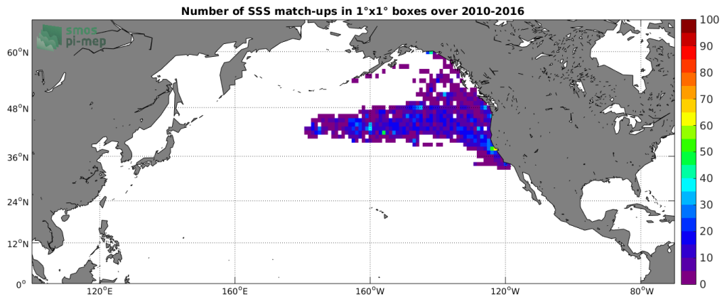
Figure 4: Number of SSS match-ups between Sea mammals SSS and the CCI SSS L4 Merged-OI v2.31 - 30-day running (ESA) SSS product for the North Pacific Ocean Pi-MEP region over 1°x1° boxes and for the full satellite product period.
