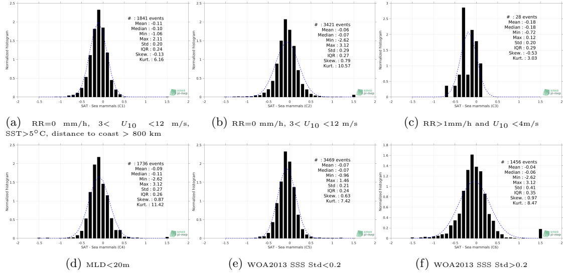
Figure 13: Normalized histogram of \Delta\text{SSS} (CCI SSS L4 Merged-OI v2.31 - 30-day running (ESA) - Sea mammals) for 6 different subdatasets corresponding to: RR=0 mm/h, 3 < U_{10} < 12 m/s, SST>5°C, distance to coast > 800 km (a), RR=0 mm/h, 3 < U_{10} < 12 m/s (b), RR>1mm/h and U_{10} < 4 m/s (c), MLD<20m (d), WOA2013 SSS Std<0.2 (e), WOA2013 SSS Std>0.2 (f).
