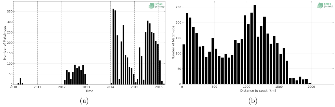
Figure 1: Number of match-ups between Sea mammals and CCI SSS L4 Merged-OI v2.31 - 30-day running (ESA) SSS as a function of time (a) and as function of the distance to coast (b) over the North Pacific Ocean Pi-MEP region and for the full satellite product period.
