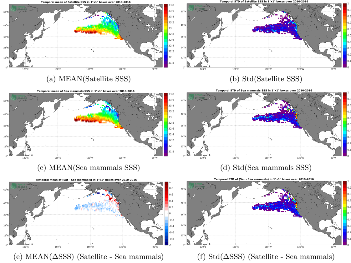
Figure 6: Temporal mean (left) and Std (right) of SSS from CCI SSS L4 Merged-OI v2.31 - 30-day running (ESA) (top), Sea mammals (middle), and of \Delta SSS (Satellite - Sea mammals). Only match-up pairs are used to generate these maps.
