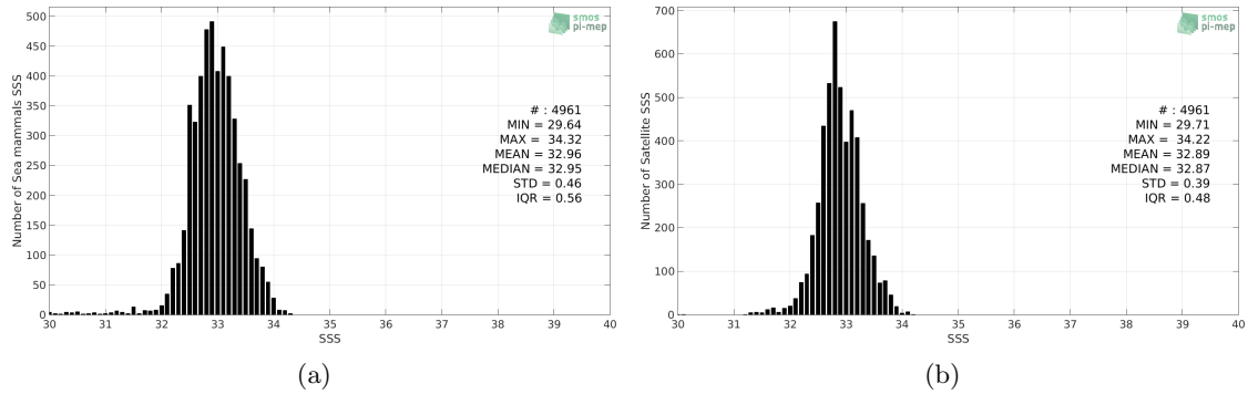
Figure 2: Histograms of SSS from Sea mammals (a) and CCI SSS L4 Merged-OI v2.31 - 30-day running (ESA) (b) considering all match-up pairs per bins of 0.1 over the North Pacific Ocean Pi-MEP region and for the full satellite product period.
