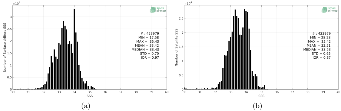
Figure 2: Histograms of SSS from Surface drifters (a) and CCI L4 Merged-OI v2.31 - 30-day running (ESA) (b) considering all match-up pairs per bins of 0.1 over the North Pacific Ocean Pi-MEP region and for the full satellite product period.
