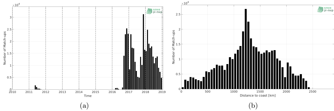
Figure 1: Number of match-ups between Surface drifters and CCI L4 Merged-OI v2.31 - 30-day running (ESA) SSS as a function of time (a) and as function of the distance to coast (b) over the North Pacific Ocean Pi-MEP region and for the full satellite product period.
