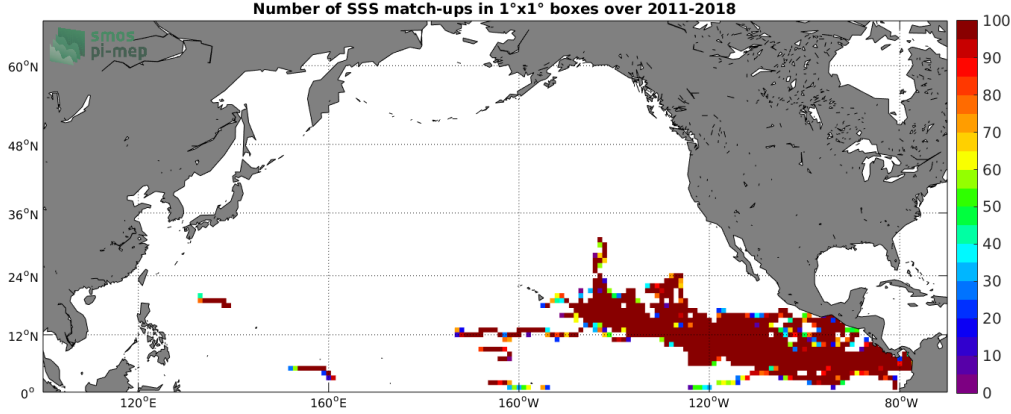
Figure 3: Number of SSS match-ups between Surface drifters SSS and the CCI L4 Merged-OI v2.31 - 30-day running (ESA) SSS product for the North Pacific Ocean Pi-MEP region over 1^\circ \times 1^\circ boxes and for the full satellite product period.
