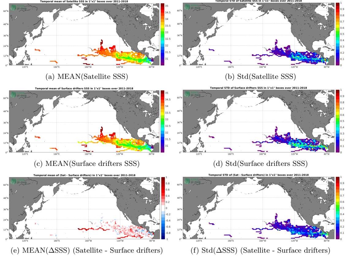
Figure 5: Temporal mean (left) and Std (right) of SSS from CCI L4 Merged-OI v2.31 - 30-day running (ESA) (top), Surface drifters (middle), and of \Delta SSS (Satellite - Surface drifters). Only match-up pairs are used to generate these maps.
