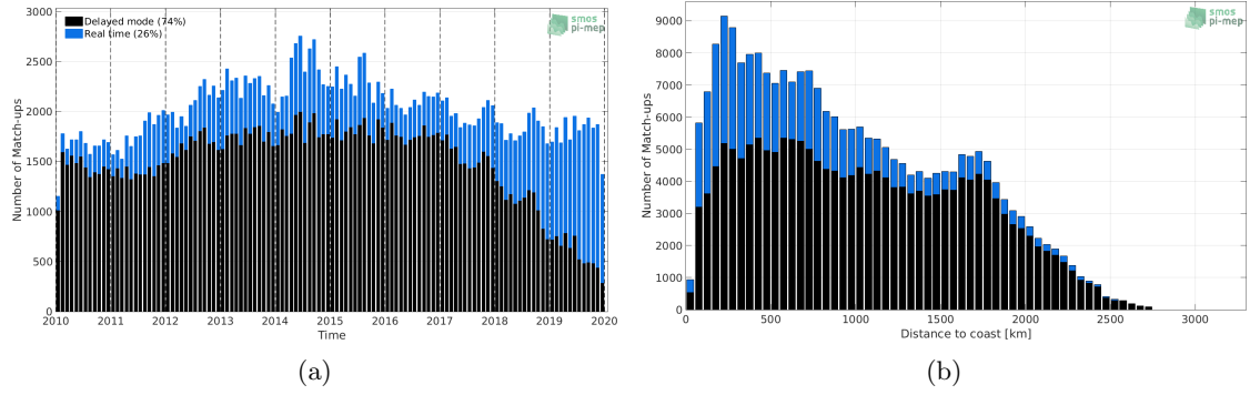
Figure 1: Number of match-ups between Argo and CCI SSS L4 Merged-OI v2.31 - 30-day running (ESA) SSS as a function of time (a) and as function of the distance to coast (b) over the North Pacific Ocean Pi-MEP region and for the full satellite product period.
