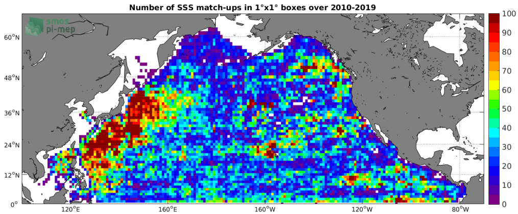
Figure 4: Number of SSS match-ups between Argo SSS and the CCI SSS L4 Merged-OI v2.31 - 30-day running (ESA) SSS product for the North Pacific Ocean Pi-MEP region over 1^\circ \times 1^\circ boxes and for the full satellite product period.
