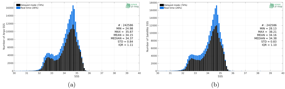
Figure 2: Histograms of SSS from Argo (a) and CCI SSS L4 Merged-OI v2.31 - 30-day running (ESA) (b) considering all match-up pairs per bins of 0.1 over the North Pacific Ocean Pi-MEP region and for the full satellite product period.
