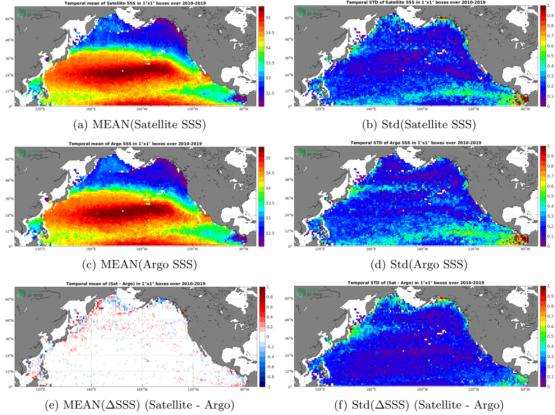
Figure 6: Temporal mean (left) and Std (right) of SSS from CCI SSS L4 Merged-OI v2.31 - 30-day running (ESA) (top), Argo (middle), and of \Delta SSS (Satellite - Argo). Only match-up pairs are used to generate these maps.
