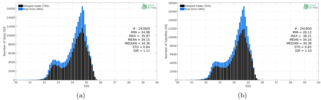
Figure 2: Histograms of SSS from Argo (a) and CCI L4 Merged-OI v2.31 - 30-day running (ESA) (b) considering all match-up pairs per bins of 0.1 over the North Pacific Ocean Pi-MEP region and for the full satellite product period.
