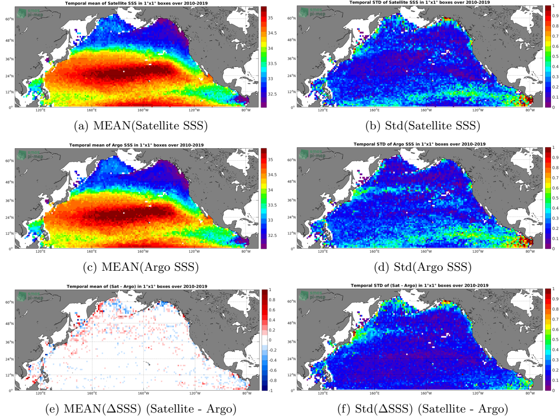
Figure 6: Temporal mean (left) and Std (right) of SSS from CCI L4 Merged-OI v2.31 - 30-day running (ESA) (top), Argo (middle), and of \Delta SSS (Satellite - Argo). Only match-up pairs are used to generate these maps.
