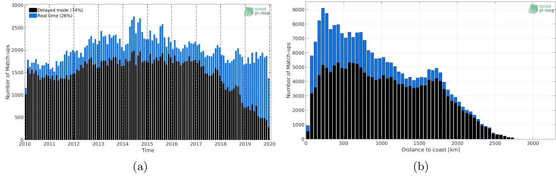
Figure 1: Number of match-ups between Argo and CCI L4 Merged-OI v2.31 - 30-day running (ESA) SSS as a function of time (a) and as function of the distance to coast (b) over the North Pacific Ocean Pi-MEP region and for the full satellite product period.
