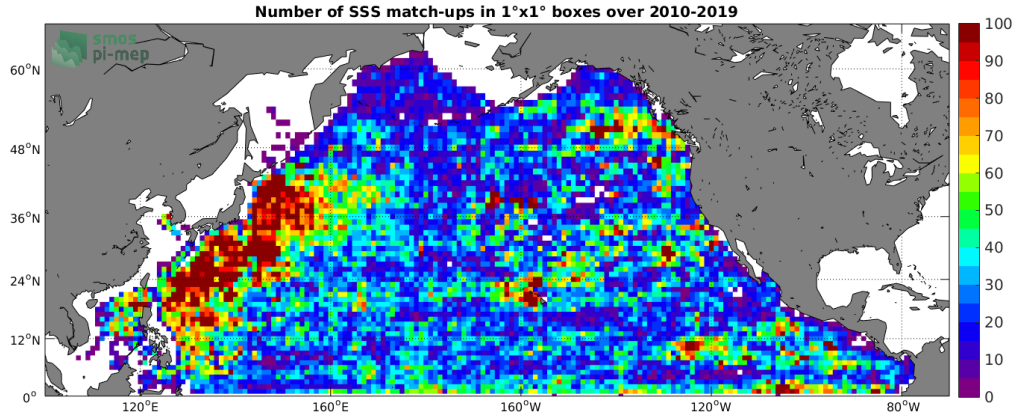
Figure 4: Number of SSS match-ups between Argo SSS and the CCI L4 Merged-OI v2.31 - 30-day running (ESA) SSS product for the North Pacific Ocean Pi-MEP region over 1^\circ \times 1^\circ boxes and for the full satellite product period.
