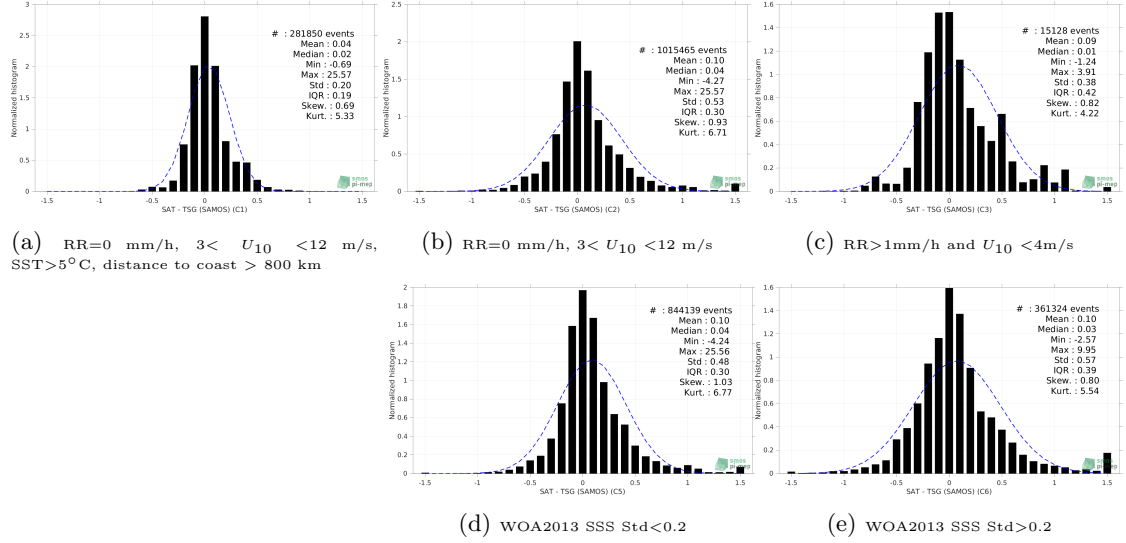
Figure 13: Normalized histogram of \Delta\text{SSS} (Aquarius SSS L4 OI v5 - Weekly (IPRC) - TSG (SAMOS)) for 5 different subdatasets corresponding to: RR=0 mm/h, 3 < U_{10} < 12 m/s, SST>5°C, distance to coast > 800 km (a), RR=0 mm/h, 3 < U_{10} < 12 m/s (b), RR>1mm/h and U_{10} < 4 m/s (c), WOA2013 SSS Std<0.2 (d), WOA2013 SSS Std>0.2 (e).
