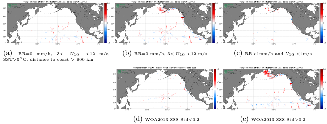
Figure 12: Temporal mean gridded over spatial boxes of size 1^\circ \times 1^\circ of \Delta SSS (Aquarius-L4-IPRC-V5-WEEKLY - TSG-SAMOS) for 5 different subdatasets corresponding to: RR=0 mm/h, 3 < U_{10} < 12 m/s, SST > 5^\circ C , distance to coast > 800 km (a), RR=0 mm/h, 3 < U_{10} < 12 m/s (b), RR > 1 mm/h and U_{10} < 4 m/s (c), WOA2013 SSS Std < 0.2 (d), WOA2013 SSS Std > 0.2 (e).
