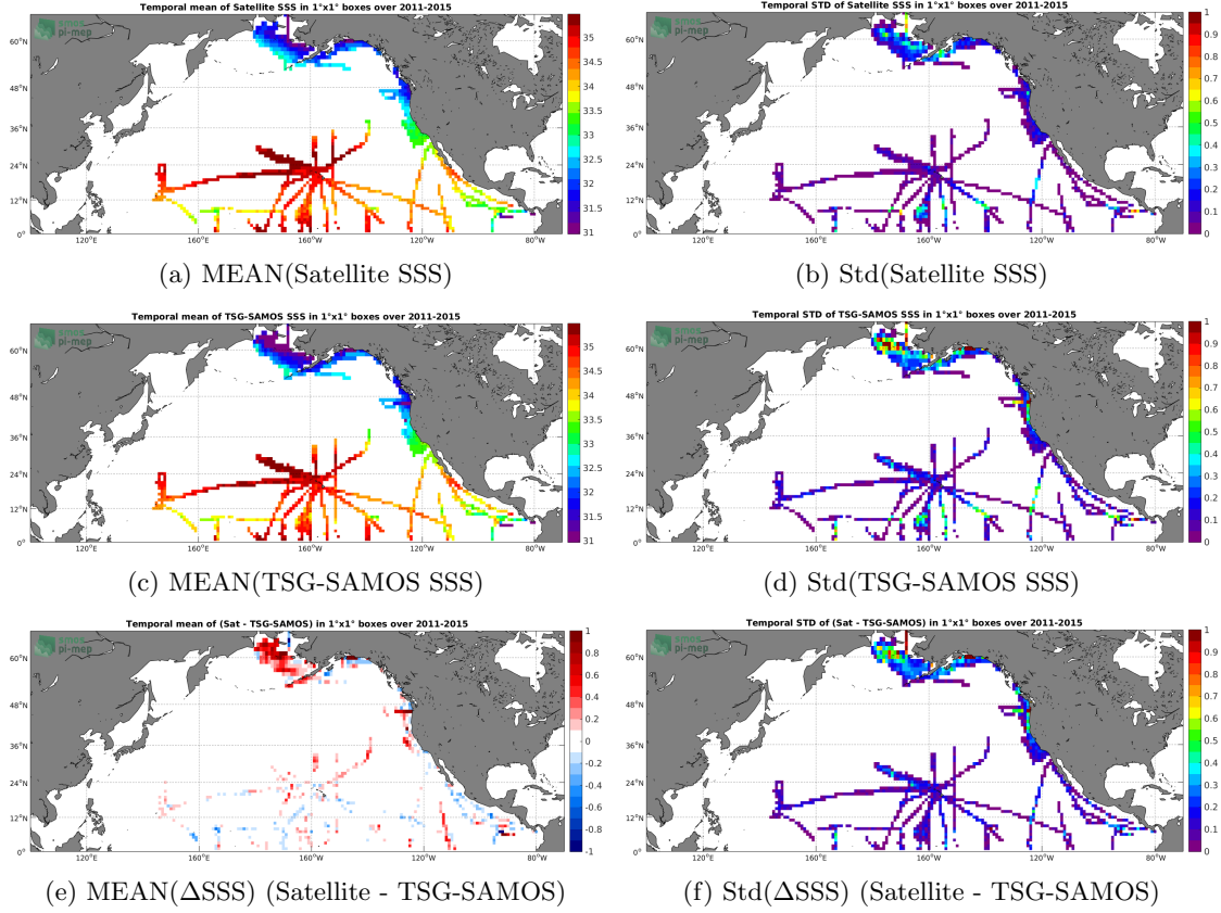
Figure 6: Temporal mean (left) and Std (right) of SSS from Aquarius-L4-IPRC-V5-WEEKLY (top), TSG-SAMOS (middle), and of \Delta SSS (Satellite - TSG-SAMOS). Only match-up pairs are used to generate these maps.
