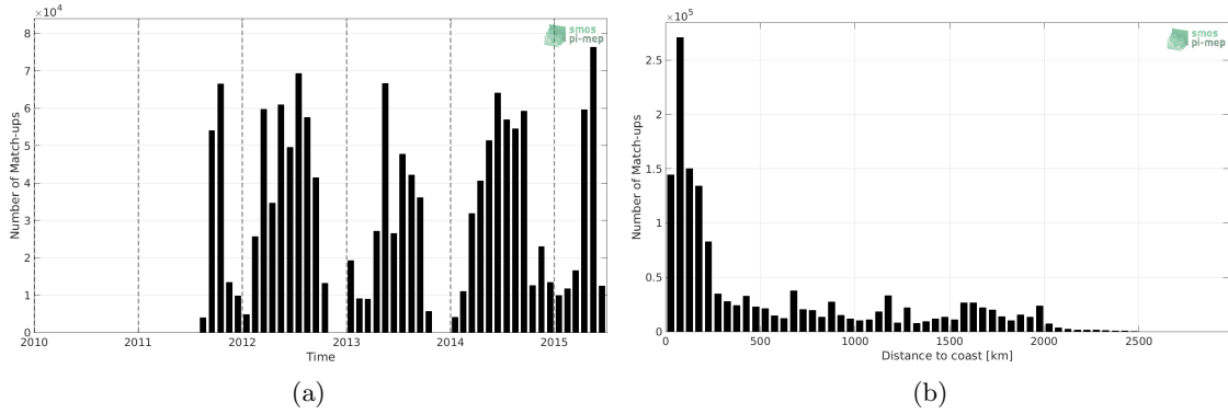
Figure 1: Number of match-ups between TSG-SAMOS and Aquarius-L4-IPRC-V5-WEEKLY SSS as a function of time (a) and as function of the distance to coast (b) over the North Pacific Ocean Pi-MEP region and for the full satellite product period.
