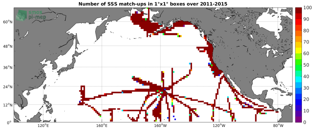
Figure 4: Number of SSS match-ups between TSG-SAMOS SSS and the Aquarius-L4-IPRC-V5-WEEKLY SSS product for the North Pacific Ocean Pi-MEP region over 1°x1° boxes and for the full satellite product period.
