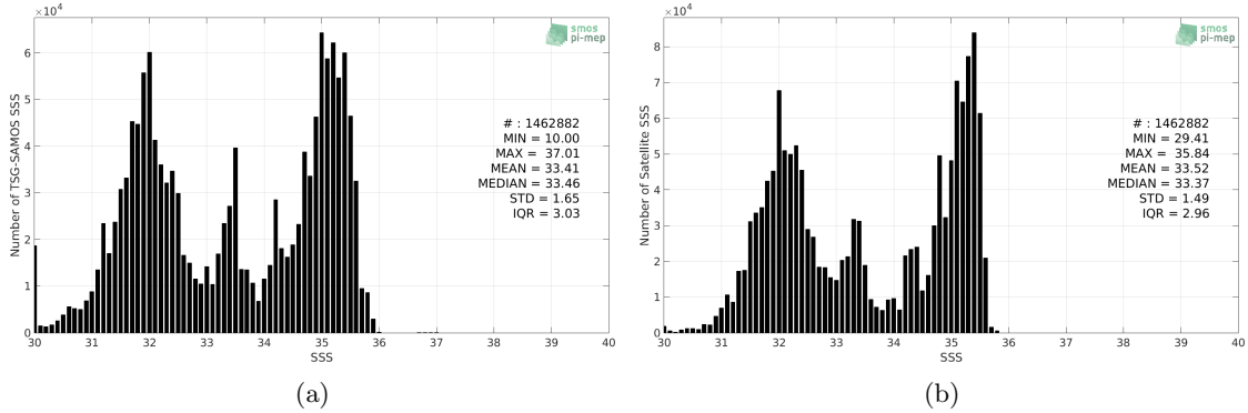
Figure 2: Histograms of SSS from TSG-SAMOS (a) and Aquarius-L4-IPRC-V5-WEEKLY (b) considering all match-up pairs per bins of 0.1 over the North Pacific Ocean Pi-MEP region and for the full satellite product period.
