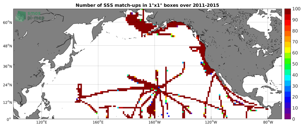
Figure 4: Number of SSS match-ups between TSG-SAMOS SSS and the Aquarius-L4-IPRC-V5-WEEKLY SSS product for the North Pacific Ocean Pi-MEP region over 1^\circ \times 1^\circ boxes and for the full satellite product period.
