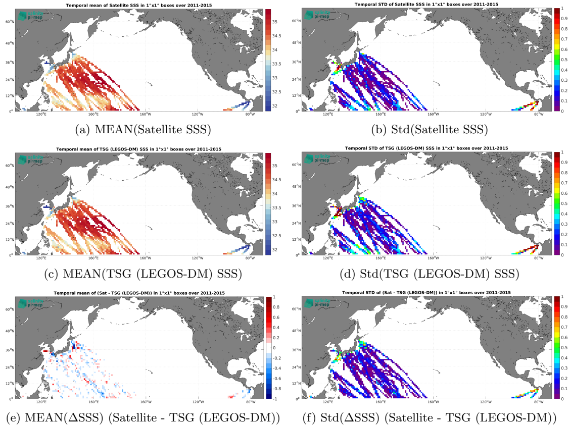
Figure 7: Temporal mean (left) and Std (right) of SSS from Aquarius SSS L4 OI v5 - Weekly (IPRC) (top), TSG (LEGOS-DM) (middle), and of \Delta SSS (Satellite - TSG (LEGOS-DM)). Only match-up pairs are used to generate these maps.
