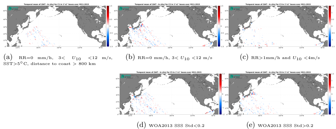
Figure 14: Temporal mean gridded over spatial boxes of size 1^\circ \times 1^\circ of \Delta\text{SSS} (Aquarius SSS L4 OI v5 - Weekly (IPRC) - TSG (LEGOS-DM)) for 5 different subdatasets corresponding to: RR=0 mm/h, 3 < U_{10} < 12 m/s, SST > 5°C, distance to coast > 800 km (a), RR=0 mm/h, 3 < U_{10} < 12 m/s (b), RR > 1 mm/h and U_{10} < 4 m/s (c), WOA2013 SSS Std < 0.2 (d), WOA2013 SSS Std > 0.2 (e).
