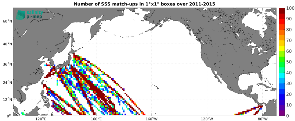
Figure 5: Number of SSS match-ups between TSG (LEGOS-DM) SSS and the Aquarius SSS L4 OI v5 - Weekly (IPRC) SSS product for the North Pacific Ocean Pi-MEP region over 1^\circ \times 1^\circ boxes and for the full satellite product period.
