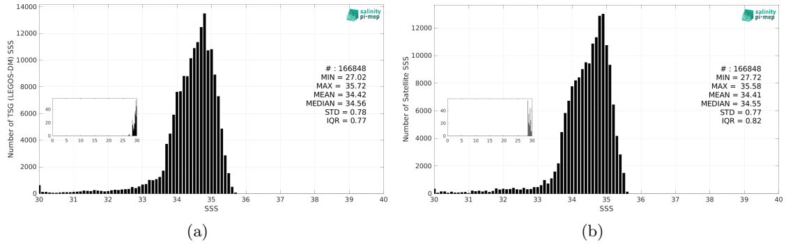
Figure 3: Histograms of SSS from TSG (LEGOS-DM) (a) and Aquarius SSS L4 OI v5 - Weekly (IPRC) (b) considering all match-up pairs per bins of 0.1 over the North Pacific Ocean Pi-MEP region and for the full satellite product period.
