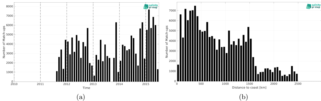
Figure 2: Number of match-ups between TSG (LEGOS-DM) and Aquarius SSS L4 OI v5 - Weekly (IPRC) SSS as a function of time (a) and as function of the distance to coast (b) over the North Pacific Ocean Pi-MEP region and for the full satellite product period.
