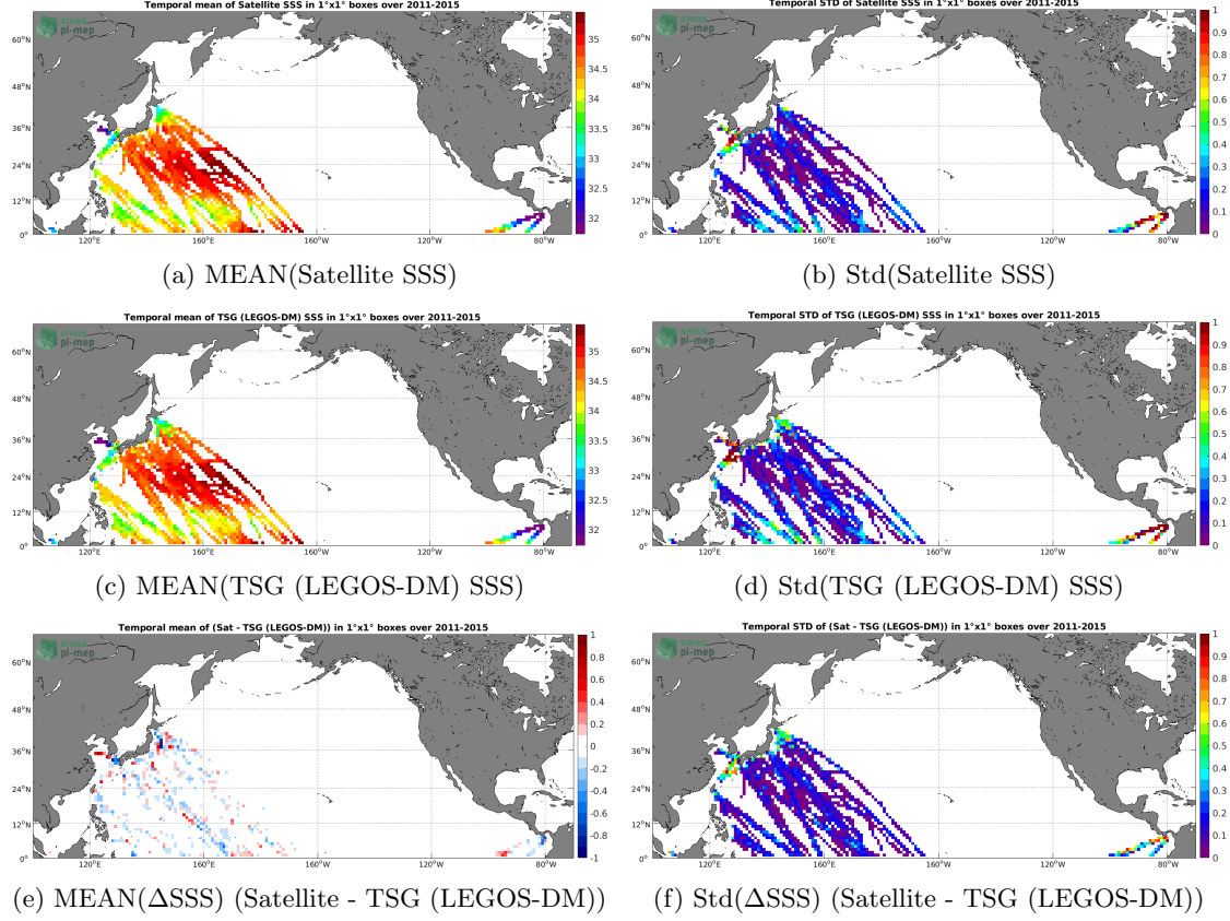
Figure 6: Temporal mean (left) and Std (right) of SSS from Aquarius SSS L4 OI v5 - Weekly (IPRC) (top), TSG (LEGOS-DM) (middle), and of \Delta\text{SSS} (Satellite - TSG (LEGOS-DM)). Only match-up pairs are used to generate these maps.
