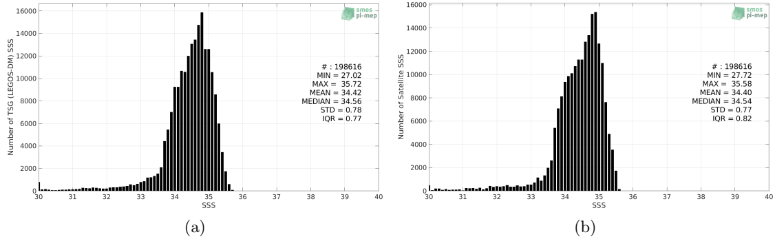
Figure 2: Histograms of SSS from TSG (LEGOS-DM) (a) and Aquarius SSS L4 OI v5 - Weekly (IPRC) (b) considering all match-up pairs per bins of 0.1 over the North Pacific Ocean Pi-MEP region and for the full satellite product period.
