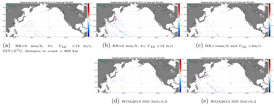
Figure 12: Temporal mean gridded over spatial boxes of size 1^\circ \times 1^\circ of \Delta SSS (Aquarius SSS L4 OI v5 - Weekly (IPRC) - TSG (LEGOS-DM)) for 5 different subdatasets corresponding to:RR=0 mm/h, 3 < U_{10} < 12 m/s, SST >5^\circ\text{C} , distance to coast > 800 km (a), RR=0 mm/h, 3 < U_{10} < 12 m/s (b), RR >1 mm/h and U_{10} < 4 m/s (c), WOA2013 SSS Std <0.2 (d), WOA2013 SSS Std >0.2 (e).
