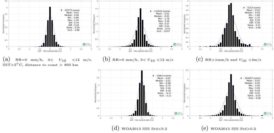
Figure 13: Normalized histogram of \Delta SSS (Aquarius SSS L4 OI v5 - Weekly (IPRC) - TSG (LEGOS-DM)) for 5 different subdatasets corresponding to: RR=0 mm/h, 3 < U_{10} < 12 m/s, SST > 5^\circ\text{C} , distance to coast > 800 km (a), RR=0 mm/h, 3 < U_{10} < 12 m/s (b), RR > 1 mm/h and U_{10} < 4 m/s (c), WOA2013 SSS Std < 0.2 (d), WOA2013 SSS Std > 0.2 (e).
