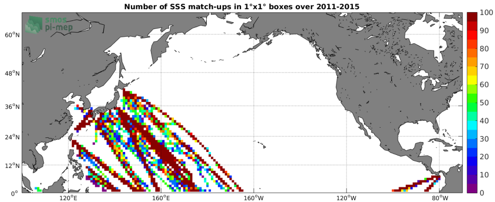
Figure 4: Number of SSS match-ups between TSG-LEGOS-DM SSS and the Aquarius-L4-IPRC-V5-WEEKLY SSS product for the North Pacific Ocean Pi-MEP region over 1°x1° boxes and for the full satellite product period.
