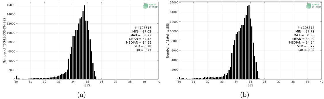
Figure 2: Histograms of SSS from TSG-LEGOS-DM (a) and Aquarius-L4-IPRC-V5-WEEKLY (b) considering all match-up pairs per bins of 0.1 over the North Pacific Ocean Pi-MEP region and for the full satellite product period.
