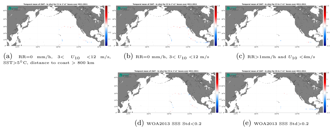
Figure 14: Temporal mean gridded over spatial boxes of size 1^\circ \times 1^\circ of \Delta\text{SSS} (Aquarius SSS L4 OI v5 - Weekly (IPRC) - TSG (GOSUD-Sailing-ship)) for 5 different subdatasets corresponding to:RR=0 mm/h, 3 < U_{10} < 12 m/s, SST>5°C, distance to coast > 800 km (a), RR=0 mm/h, 3 < U_{10} < 12 m/s (b), RR>1mm/h and U_{10} < 4 m/s (c), WOA2013 SSS Std<0.2 (d), WOA2013 SSS Std>0.2 (e).
