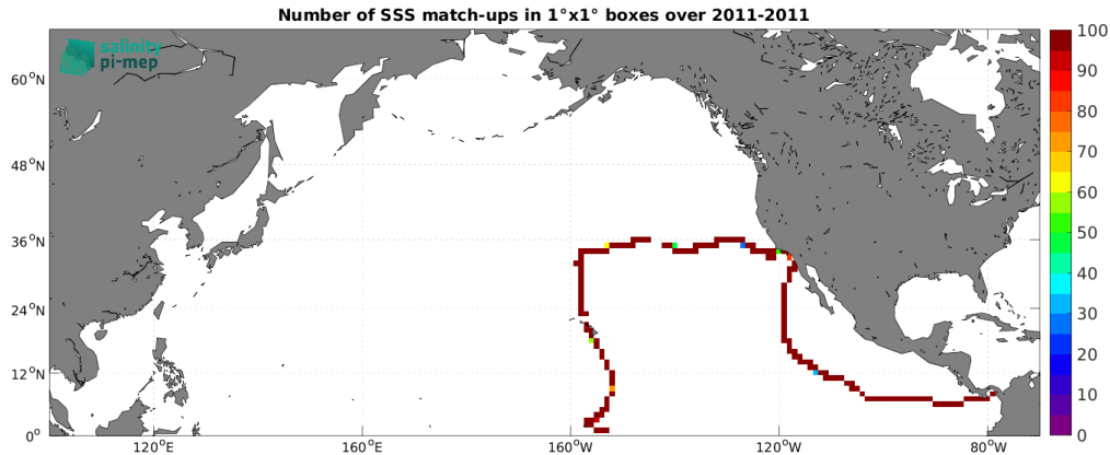
Figure 5: Number of SSS match-ups between TSG (GOSUD-Sailing-ship) SSS and the Aquarius SSS L4 OI v5 - Weekly (IPRC) SSS product for the North Pacific Ocean Pi-MEP region over 1^\circ \times 1^\circ boxes and for the full satellite product period.
