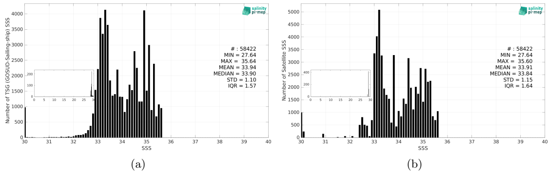
Figure 3: Histograms of SSS from TSG (GOSUD-Sailing-ship) (a) and Aquarius SSS L4 OI v5 - Weekly (IPRC) (b) considering all match-up pairs per bins of 0.1 over the North Pacific Ocean Pi-MEP region and for the full satellite product period.
