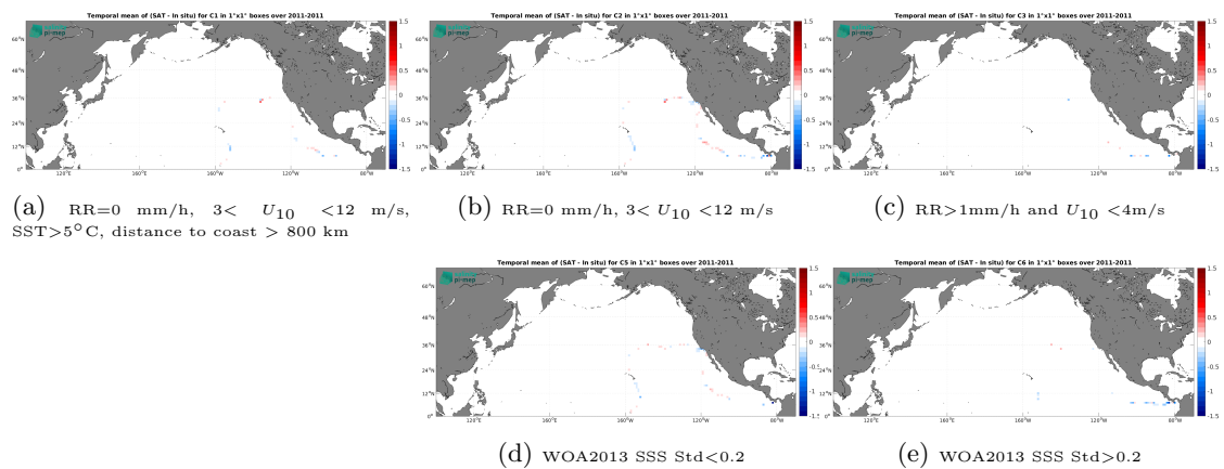
Figure 12: Temporal mean gridded over spatial boxes of size 1^\circ \times 1^\circ of \Delta\text{SSS} (Aquarius SSS L4 OI v5 - Weekly (IPRC) - TSG (GOSUD-Sailing-ship)) for 5 different subdatasets corresponding to:RR=0 mm/h, 3 < U_{10} < 12 m/s, SST >5^\circ\text{C} , distance to coast > 800 km (a), RR=0 mm/h, 3 < U_{10} < 12 m/s (b), RR >1 mm/h and U_{10} < 4 m/s (c), WOA2013 SSS Std <0.2 (d), WOA2013 SSS Std >0.2 (e).
