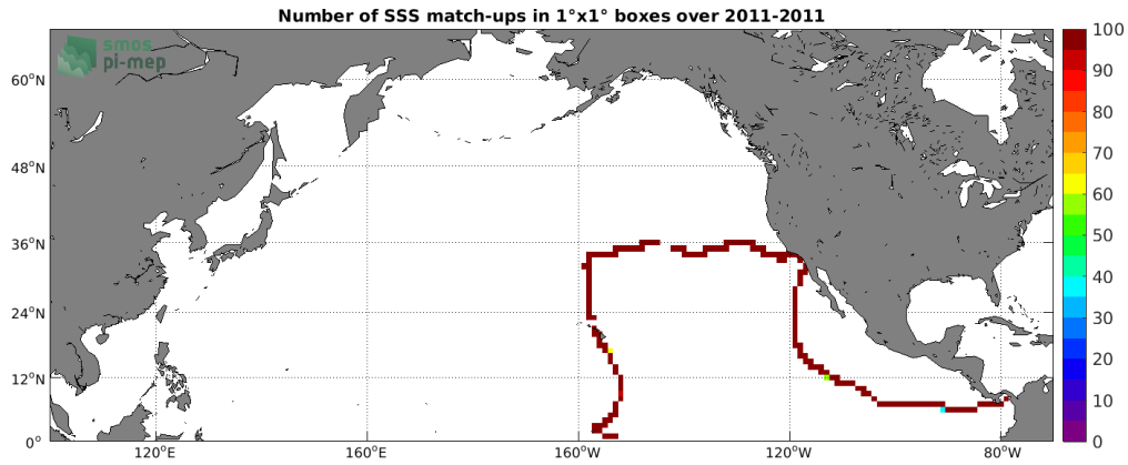
Figure 4: Number of SSS match-ups between TSG (GOSUD-Sailing-ship) SSS and the Aquarius SSS L4 OI v5 - Weekly (IPRC) SSS product for the North Pacific Ocean Pi-MEP region over 1^\circ \times 1^\circ boxes and for the full satellite product period.
