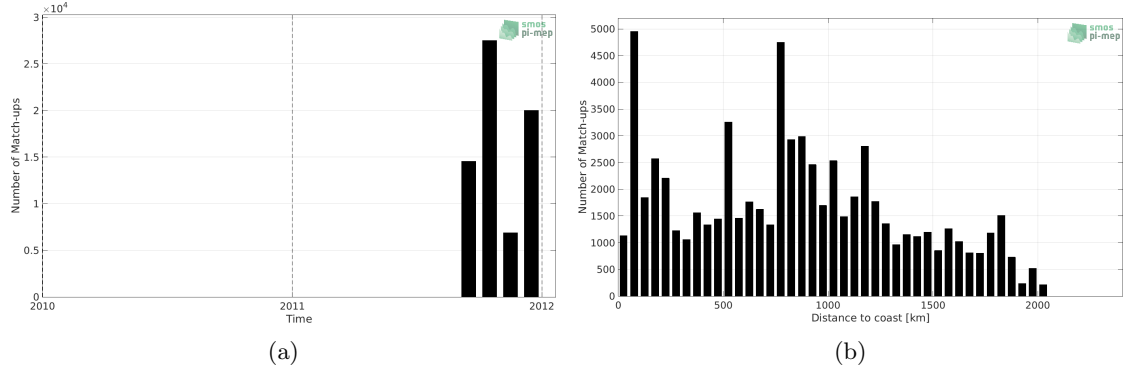
Figure 1: Number of match-ups between TSG (GOSUD-Sailing-ship) and Aquarius SSS L4 OI v5 - Weekly (IPRC) SSS as a function of time (a) and as function of the distance to coast (b) over the North Pacific Ocean Pi-MEP region and for the full satellite product period.
