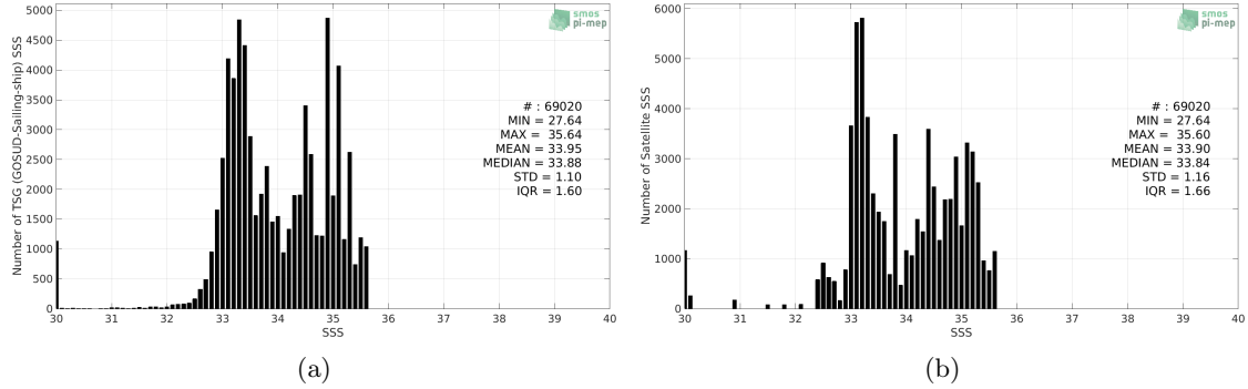
Figure 2: Histograms of SSS from TSG (GOSUD-Sailing-ship) (a) and Aquarius SSS L4 OI v5 - Weekly (IPRC) (b) considering all match-up pairs per bins of 0.1 over the North Pacific Ocean Pi-MEP region and for the full satellite product period.
