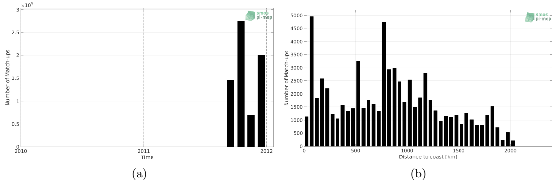
Figure 1: Number of match-ups between TSG-GOSUD-Sailing-ship and Aquarius-L4-IPRC-V5-WEEKLY SSS as a function of time (a) and as function of the distance to coast (b) over the North Pacific Ocean Pi-MEP region and for the full satellite product period.
