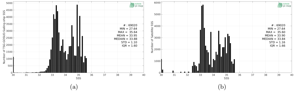
Figure 2: Histograms of SSS from TSG-GOSUD-Sailing-ship (a) and Aquarius-L4-IPRC-V5-WEEKLY (b) considering all match-up pairs per bins of 0.1 over the North Pacific Ocean Pi-MEP region and for the full satellite product period.
