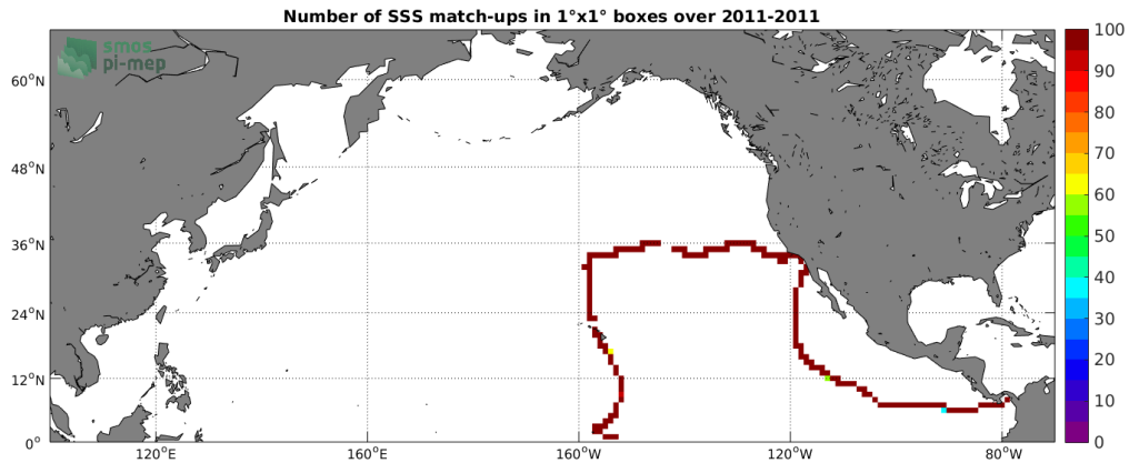
Figure 4: Number of SSS match-ups between TSG-GOSUD-Sailing-ship SSS and the Aquarius-L4-IPRC-V5-WEEKLY SSS product for the North Pacific Ocean Pi-MEP region over 1^\circ \times 1^\circ boxes and for the full satellite product period.
