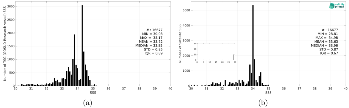
Figure 3: Histograms of SSS from TSG (GOSUD-Research-vessel) (a) and Aquarius SSS L4 OI v5 - Weekly (IPRC) (b) considering all match-up pairs per bins of 0.1 over the North Pacific Ocean Pi-MEP region and for the full satellite product period.
