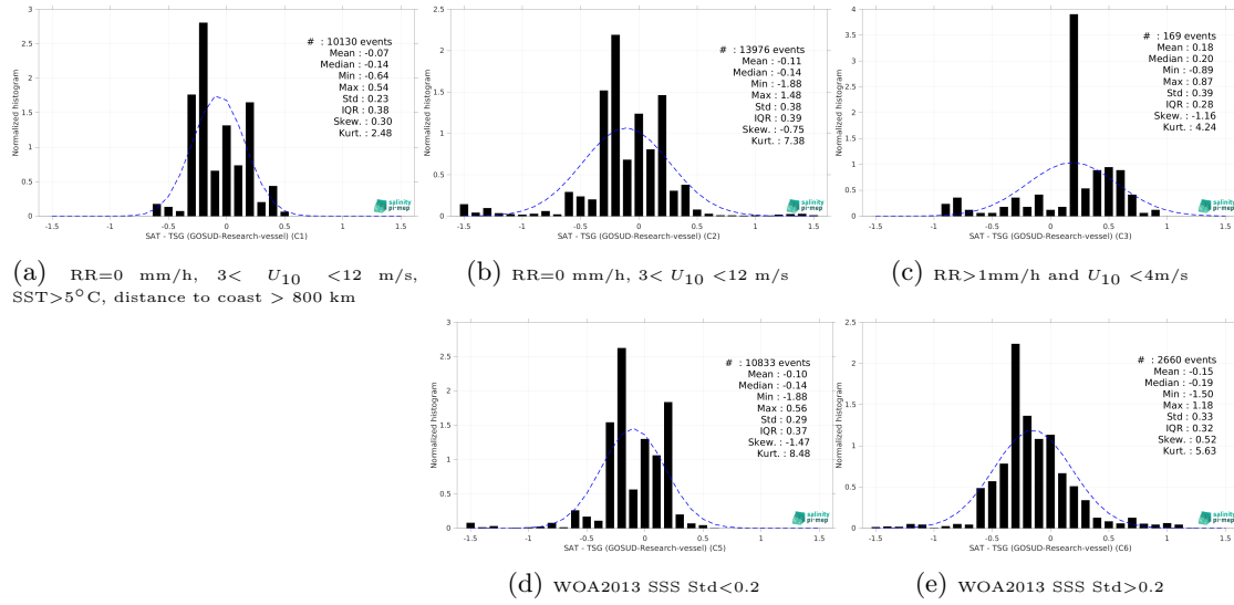
Figure 15: Normalized histogram of \Delta\text{SSS} (Aquarius SSS L4 OI v5 - Weekly (IPRC) - TSG (GOSUD-Research-vessel)) for 5 different subdatasets corresponding to: RR=0 mm/h, 3 < U_{10} < 12 m/s, SST > 5^\circ\text{C} , distance to coast > 800 km (a), RR=0 mm/h, 3 < U_{10} < 12 m/s (b), RR > 1 mm/h and U_{10} < 4 m/s (c), WOA2013 SSS Std < 0.2 (d), WOA2013 SSS Std > 0.2 (e).
