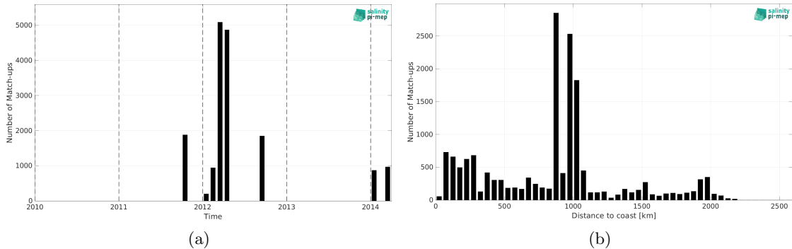
Figure 2: Number of match-ups between TSG (GOSUD-Research-vessel) and Aquarius SSS L4 OI v5 - Weekly (IPRC) SSS as a function of time (a) and as function of the distance to coast (b) over the North Pacific Ocean Pi-MEP region and for the full satellite product period.
