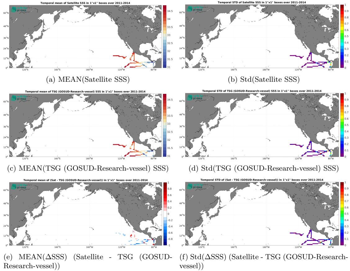
Figure 7: Temporal mean (left) and Std (right) of SSS from Aquarius SSS L4 OI v5 - Weekly (IPRC) (top), TSG (GOSUD-Research-vessel) (middle), and of \Delta SSS (Satellite - TSG (GOSUD-Research-vessel)). Only match-up pairs are used to generate these maps.
