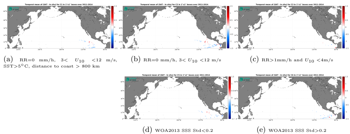
Figure 14: Temporal mean gridded over spatial boxes of size 1^\circ \times 1^\circ of \Delta SSS (Aquarius SSS L4 OI v5 - Weekly (IPRC) - TSG (GOSUD-Research-vessel)) for 5 different subdatasets corresponding to: RR=0 mm/h, 3 < U_{10} < 12 m/s, SST > 5°C, distance to coast > 800 km (a), RR=0 mm/h, 3 < U_{10} < 12 m/s (b), RR > 1 mm/h and U_{10} < 4 m/s (c), WOA2013 SSS Std < 0.2 (d), WOA2013 SSS Std > 0.2 (e).
