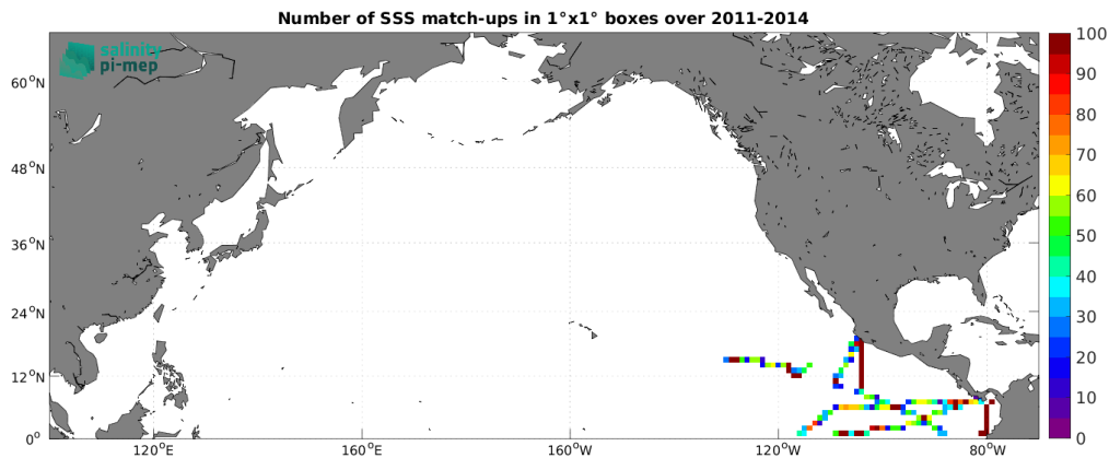
Figure 5: Number of SSS match-ups between TSG (GOSUD-Research-vessel) SSS and the Aquarius SSS L4 OI v5 - Weekly (IPRC) SSS product for the North Pacific Ocean Pi-MEP region over 1^\circ \times 1^\circ boxes and for the full satellite product period.
