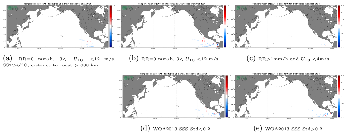
Figure 12: Temporal mean gridded over spatial boxes of size 1^\circ \times 1^\circ of \Delta SSS (Aquarius SSS L4 OI v5 - Weekly (IPRC) - TSG (GOSUD-Research-vessel)) for 5 different subdatasets corresponding to:RR=0 mm/h, 3 < U_{10} < 12 m/s, SST>5°C, distance to coast > 800 km (a), RR=0 mm/h, 3 < U_{10} < 12 m/s (b), RR>1mm/h and U_{10} < 4 m/s (c), WOA2013 SSS Std<0.2 (d), WOA2013 SSS Std>0.2 (e).
