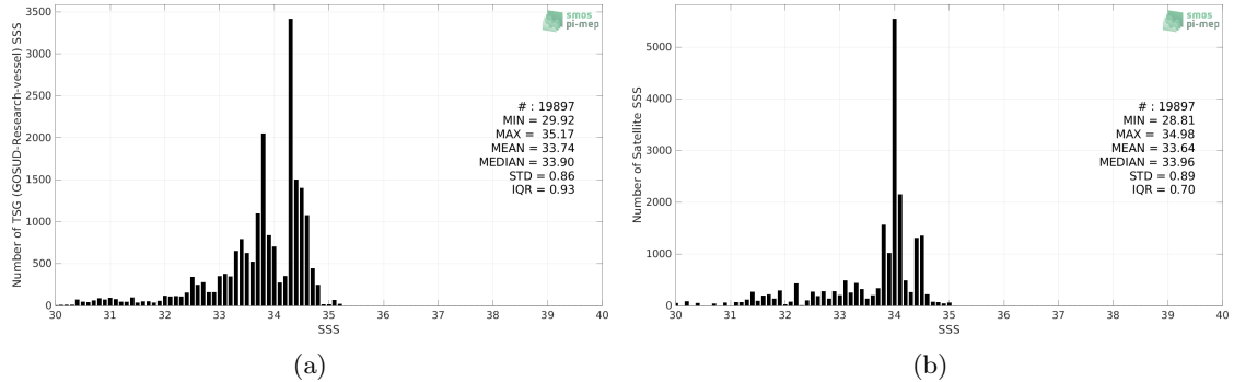
Figure 2: Histograms of SSS from TSG (GOSUD-Research-vessel) (a) and Aquarius SSS L4 OI v5 - Weekly (IPRC) (b) considering all match-up pairs per bins of 0.1 over the North Pacific Ocean Pi-MEP region and for the full satellite product period.
