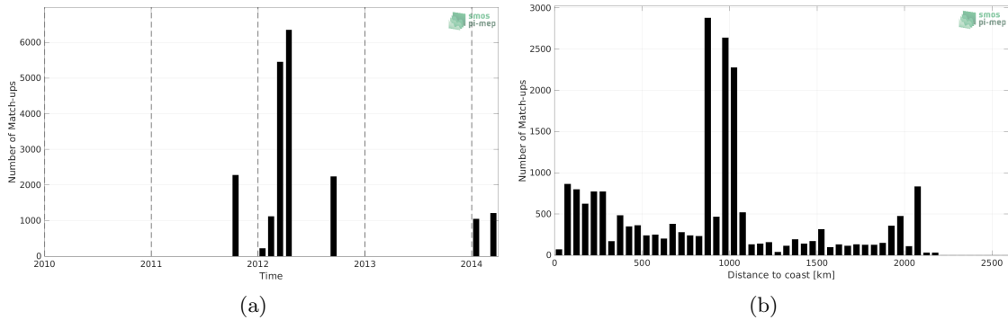
Figure 1: Number of match-ups between TSG (GOSUD-Research-vessel) and Aquarius SSS L4 OI v5 - Weekly (IPRC) SSS as a function of time (a) and as function of the distance to coast (b) over the North Pacific Ocean Pi-MEP region and for the full satellite product period.
