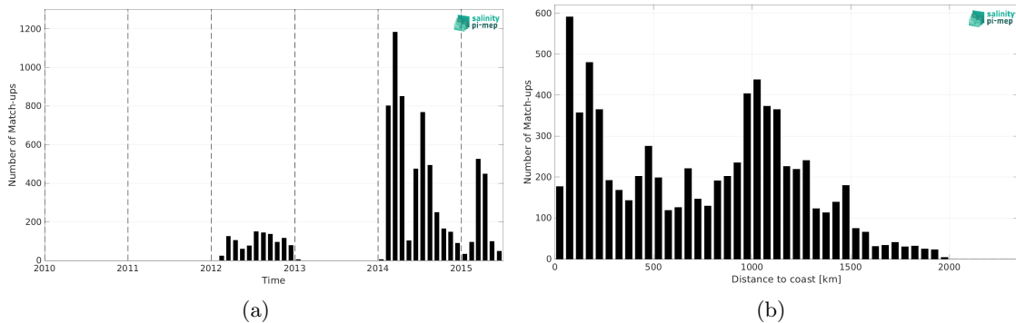
Figure 2: Number of match-ups between Marine mammals and Aquarius SSS L4 OI v5 - Weekly (IPRC) SSS as a function of time (a) and as function of the distance to coast (b) over the North Pacific Ocean Pi-MEP region and for the full satellite product period.
