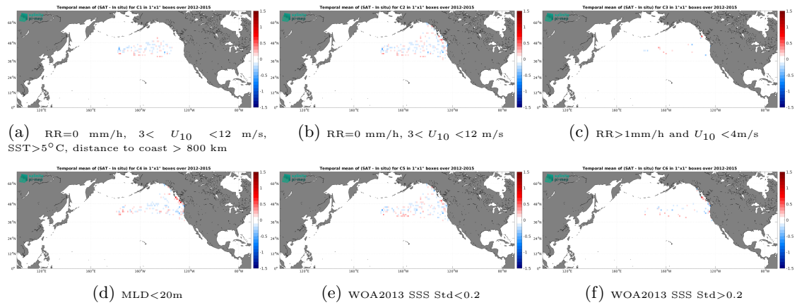
Figure 14: Temporal mean gridded over spatial boxes of size 1^\circ \times 1^\circ of \Delta SSS (Aquarius SSS L4 OI v5 - Weekly (IPRC) - Marine mammals) for 6 different subdatasets corresponding to:RR=0 mm/h, 3 < U_{10} < 12 m/s, SST>5°C, distance to coast > 800 km (a), RR=0 mm/h, 3 < U_{10} < 12 m/s (b), RR>1mm/h and U_{10} < 4 m/s (c),MLD<20m (d),WOA2013 SSS Std<0.2 (e),WOA2013 SSS Std>0.2 (f).
