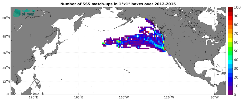
Figure 5: Number of SSS match-ups between Marine mammals SSS and the Aquarius SSS L4 OI v5 - Weekly (IPRC) SSS product for the North Pacific Ocean Pi-MEP region over 1^\circ \times 1^\circ boxes and for the full satellite product period.
