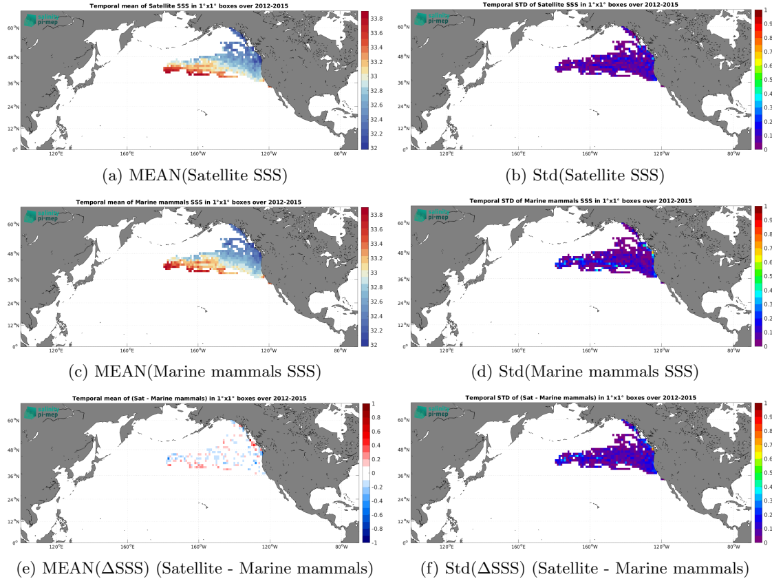
Figure 7: Temporal mean (left) and Std (right) of SSS from Aquarius SSS L4 OI v5 - Weekly (IPRC) (top), Marine mammals (middle), and of \Delta SSS (Satellite - Marine mammals). Only match-up pairs are used to generate these maps.
