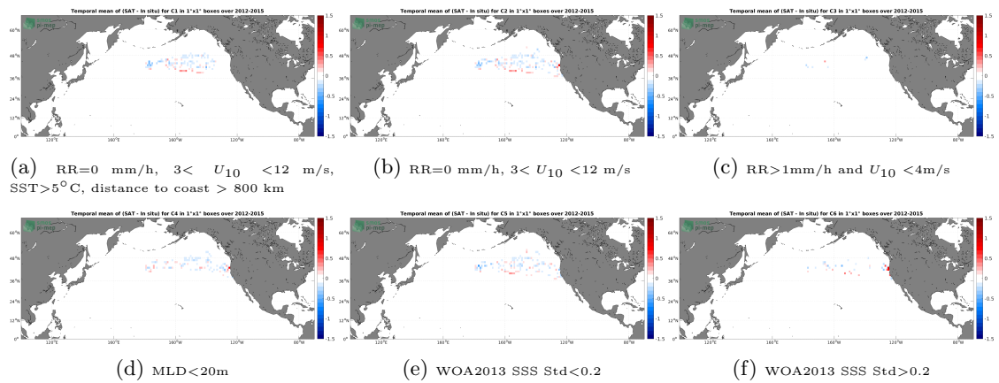
Figure 12: Temporal mean gridded over spatial boxes of size 1^\circ \times 1^\circ of \Delta SSS (Aquarius SSS L4 OI v5 - Weekly (IPRC) - Marine mammals) for 6 different subdatasets corresponding to:RR=0 mm/h, 3 < U_{10} < 12 m/s, SST >5^\circ C, distance to coast > 800 km (a), RR=0 mm/h, 3 < U_{10} < 12 m/s (b), RR >1 mm/h and U_{10} < 4 m/s (c),MLD <20 m (d),WOA2013 SSS Std <0.2 (e),WOA2013 SSS Std >0.2 (f).
