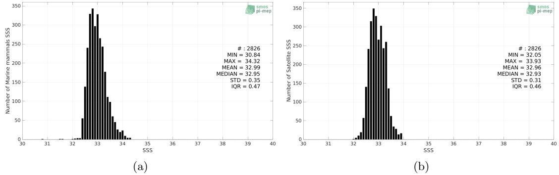
Figure 2: Histograms of SSS from Marine mammals (a) and Aquarius SSS L4 OI v5 - Weekly (IPRC) (b) considering all match-up pairs per bins of 0.1 over the North Pacific Ocean Pi-MEP region and for the full satellite product period.
