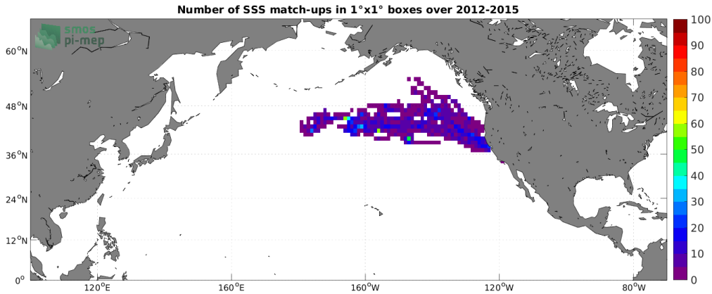
Figure 4: Number of SSS match-ups between Marine mammals SSS and the Aquarius SSS L4 OI v5 - Weekly (IPRC) SSS product for the North Pacific Ocean Pi-MEP region over 1^\circ \times 1^\circ boxes and for the full satellite product period.
