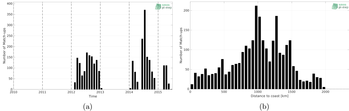
Figure 1: Number of match-ups between Marine mammals and Aquarius SSS L4 OI v5 - Weekly (IPRC) SSS as a function of time (a) and as function of the distance to coast (b) over the North Pacific Ocean Pi-MEP region and for the full satellite product period.
