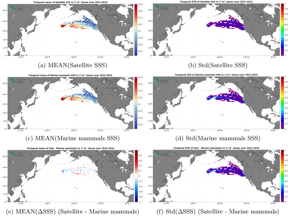
Figure 6: Temporal mean (left) and Std (right) of SSS from Aquarius SSS L4 OI v5 - Weekly (IPRC) (top), Marine mammals (middle), and of \Delta SSS (Satellite - Marine mammals). Only match-up pairs are used to generate these maps.
