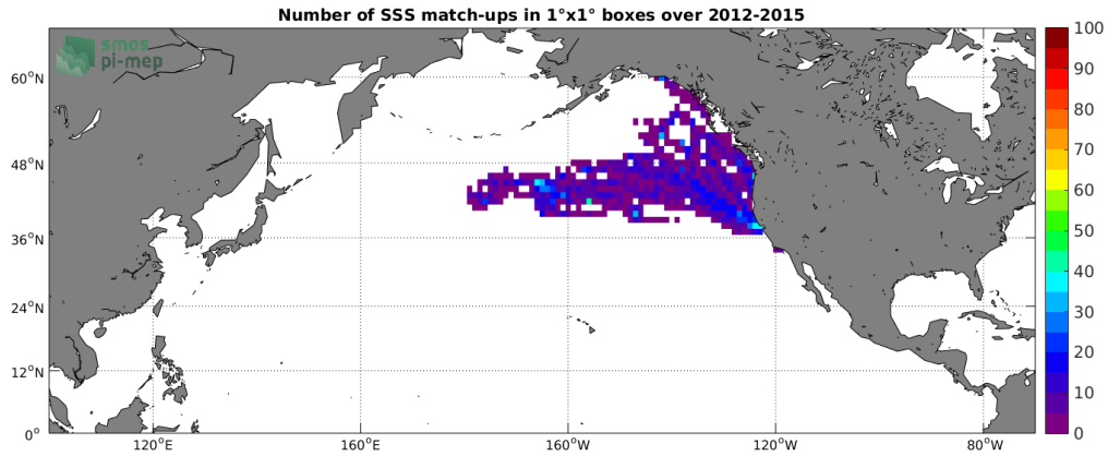
Figure 4: Number of SSS match-ups between Sea mammals SSS and the Aquarius-L4-IPRC-V5-WEEKLY SSS product for the North Pacific Ocean Pi-MEP region over 1^\circ \times 1^\circ boxes and for the full satellite product period.
