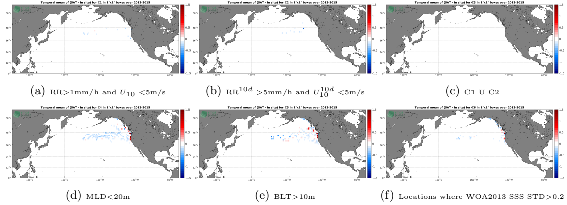
Figure 12: Temporal mean gridded over spatial boxes of size 1^\circ \times 1^\circ of \Delta SSS (Aquarius-L4-IPRC-V5-WEEKLY - Sea mammals) for 6 different subdatasets corresponding to: RR > 1\text{mm/h} and U_{10} < 5\text{m/s} (a), RR^{10d} > 5\text{mm/h} and U_{10}^{10d} < 5\text{m/s} (b), C1 U C2 (c), MLD < 20\text{m} (d), BLT > 10\text{m} (e), Locations where WOA2013 SSS STD > 0.2 (f).
