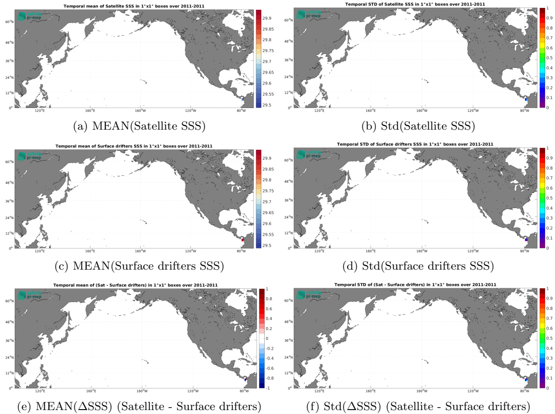
Figure 6: Temporal mean (left) and Std (right) of SSS from Aquarius SSS L4 OI v5 - Weekly (IPRC) (top), Surface drifters (middle), and of \Delta SSS (Satellite - Surface drifters). Only match-up pairs are used to generate these maps.
