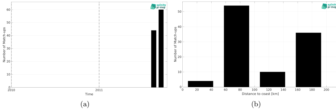
Figure 2: Number of match-ups between Surface drifters and Aquarius SSS L4 OI v5 - Weekly (IPRC) SSS as a function of time (a) and as function of the distance to coast (b) over the North Pacific Ocean Pi-MEP region and for the full satellite product period.
