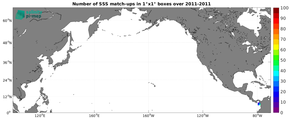
Figure 4: Number of SSS match-ups between Surface drifters SSS and the Aquarius SSS L4 OI v5 - Weekly (IPRC) SSS product for the North Pacific Ocean Pi-MEP region over 1^\circ \times 1^\circ boxes and for the full satellite product period.
