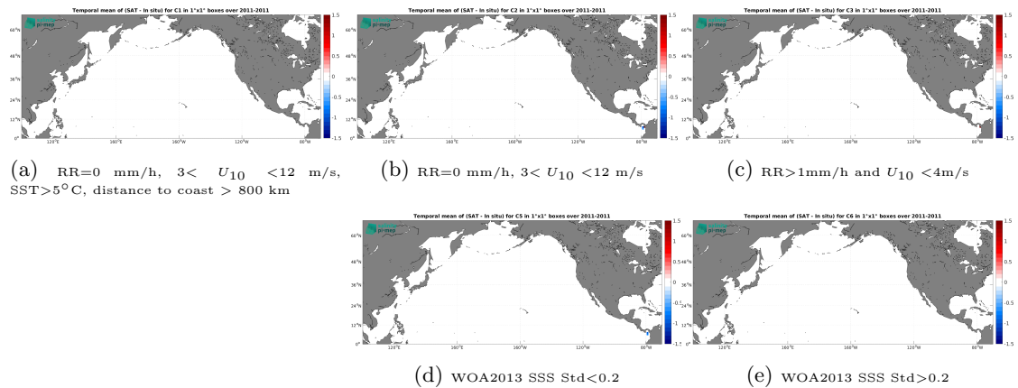
Figure 13: Temporal mean gridded over spatial boxes of size 1^\circ \times 1^\circ of \Delta SSS (Aquarius SSS L4 OI v5 - Weekly (IPRC) - Surface drifters) for 5 different subdatasets corresponding to:RR=0 mm/h, 3 < U_{10} < 12 m/s, SST>5°C, distance to coast > 800 km (a), RR=0 mm/h, 3 < U_{10} < 12 m/s (b), RR>1mm/h and U_{10} < 4 m/s (c), WOA2013 SSS Std<0.2 (d), WOA2013 SSS Std>0.2 (e).
