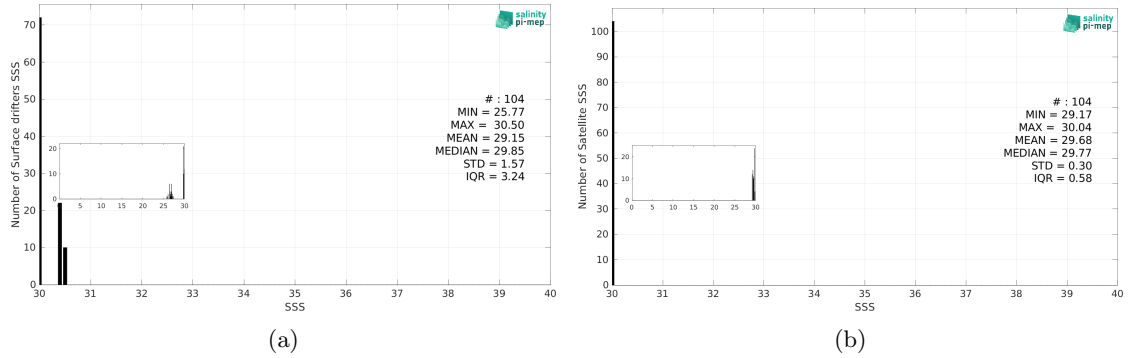
Figure 3: Histograms of SSS from Surface drifters (a) and Aquarius SSS L4 OI v5 - Weekly (IPRC) (b) considering all match-up pairs per bins of 0.1 over the North Pacific Ocean Pi-MEP region and for the full satellite product period.
