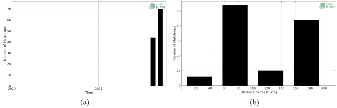
Figure 1: Number of match-ups between Surface drifters and Aquarius SSS L4 OI v5 - Weekly (IPRC) SSS as a function of time (a) and as function of the distance to coast (b) over the North Pacific Ocean Pi-MEP region and for the full satellite product period.
