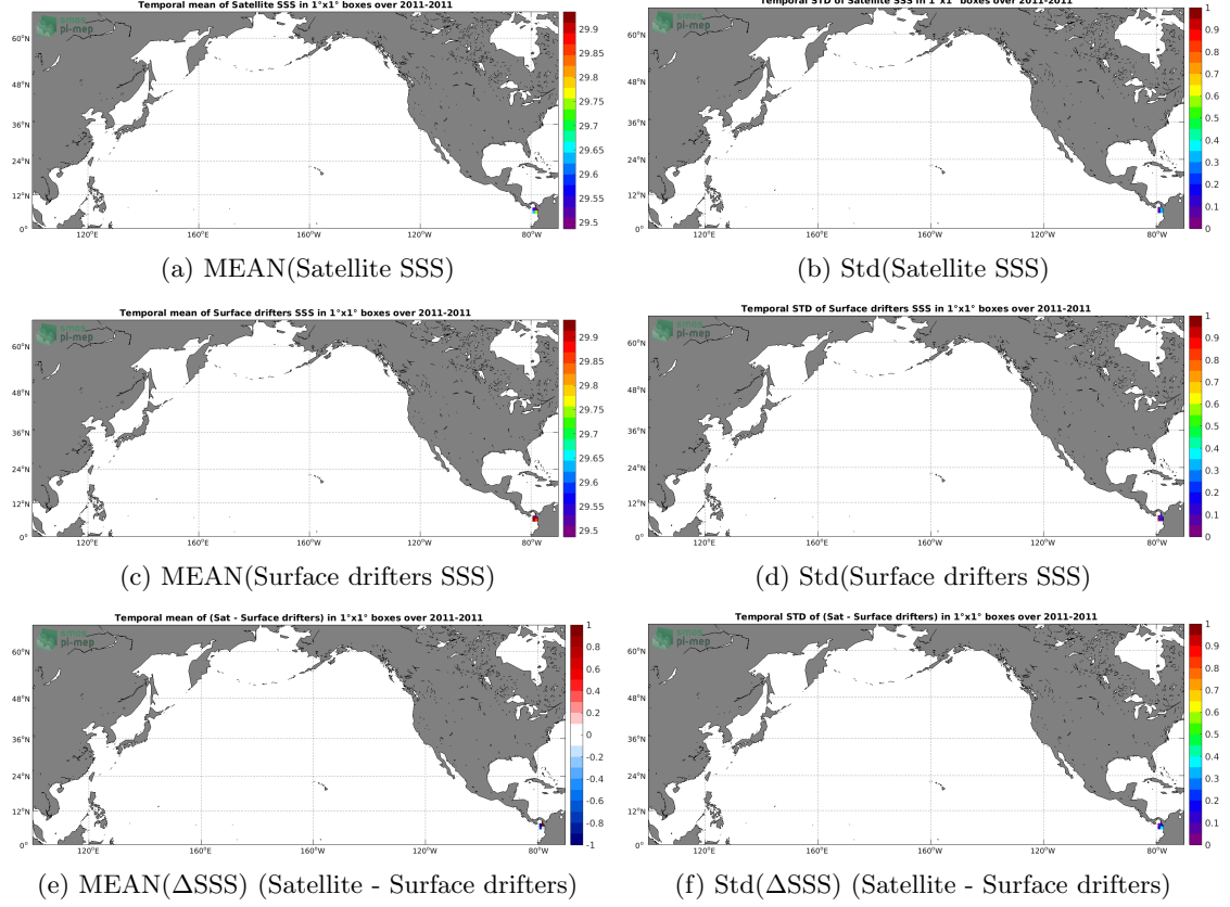
Figure 5: Temporal mean (left) and Std (right) of SSS from Aquarius SSS L4 OI v5 - Weekly (IPRC) (top), Surface drifters (middle), and of \Delta SSS (Satellite - Surface drifters). Only match-up pairs are used to generate these maps.
