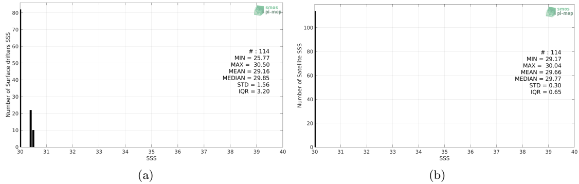
Figure 2: Histograms of SSS from Surface drifters (a) and Aquarius SSS L4 OI v5 - Weekly (IPRC) (b) considering all match-up pairs per bins of 0.1 over the North Pacific Ocean Pi-MEP region and for the full satellite product period.
