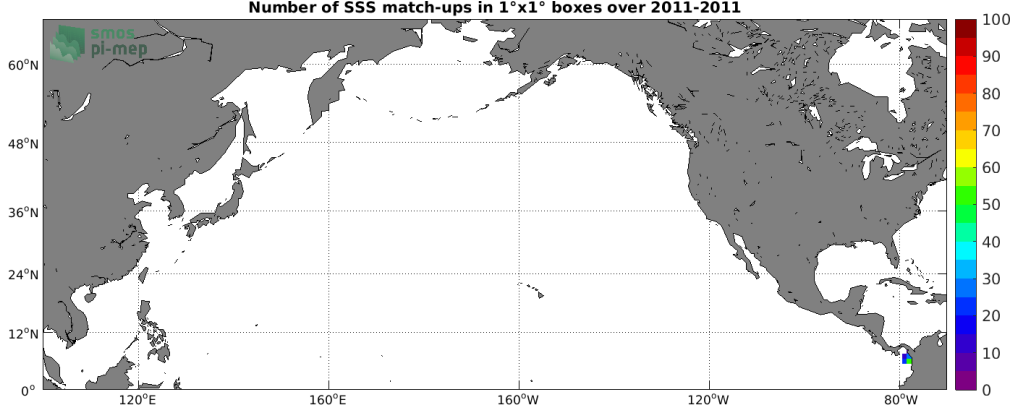
Figure 3: Number of SSS match-ups between Surface drifters SSS and the Aquarius SSS L4 OI v5 - Weekly (IPRC) SSS product for the North Pacific Ocean Pi-MEP region over 1^\circ \times 1^\circ boxes and for the full satellite product period.
