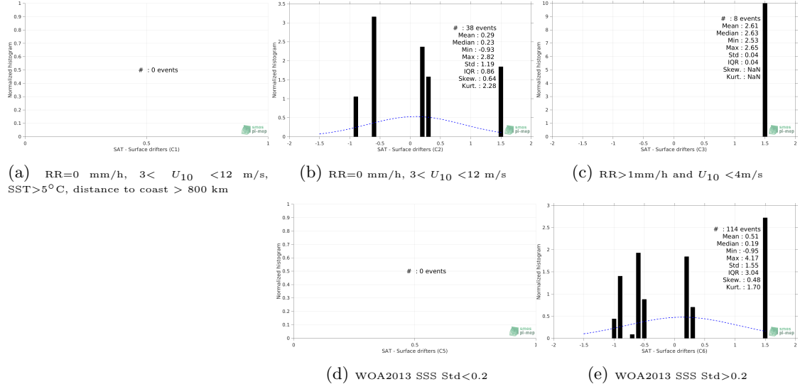
Figure 12: Normalized histogram of \Delta\text{SSS} (Aquarius SSS L4 OI v5 - Weekly (IPRC) - Surface drifters) for 5 different subdatasets corresponding to: RR=0 mm/h, 3 < U_{10} < 12 m/s, SST > 5^\circ\text{C} , distance to coast > 800 km (a), RR=0 mm/h, 3 < U_{10} < 12 m/s (b), RR > 1 mm/h and U_{10} < 4 m/s (c), WOA2013 SSS Std < 0.2 (d), WOA2013 SSS Std > 0.2 (e).
