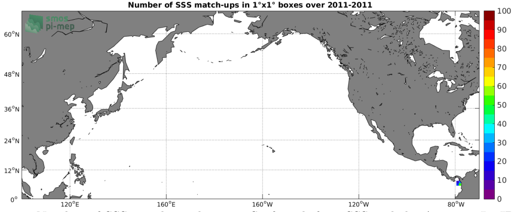
Figure 3: Number of SSS match-ups between Surface drifters SSS and the Aquarius-L4-IPRC-V5-WEEKLY SSS product for the North Pacific Ocean Pi-MEP region over 1^\circ \times 1^\circ boxes and for the full satellite product period.
