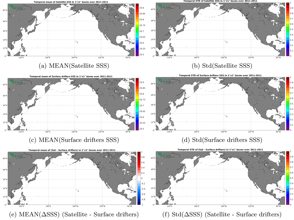
Figure 5: Temporal mean (left) and Std (right) of SSS from Aquarius-L4-IPRC-V5-WEEKLY (top), Surface drifters (middle), and of \Delta SSS (Satellite - Surface drifters). Only match-up pairs are used to generate these maps.
