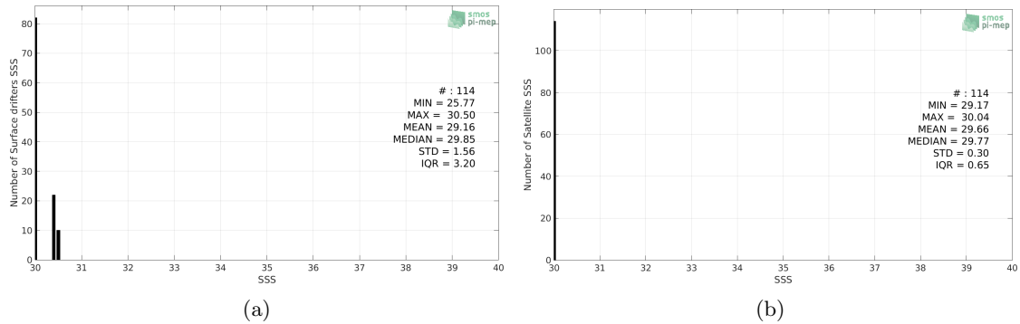
Figure 2: Histograms of SSS from Surface drifters (a) and Aquarius-L4-IPRC-V5-WEEKLY (b) considering all match-up pairs per bins of 0.1 over the North Pacific Ocean Pi-MEP region and for the full satellite product period.
