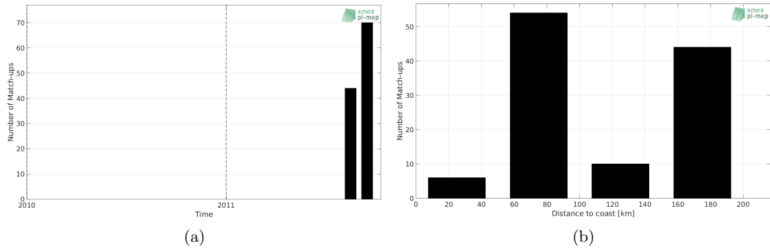
Figure 1: Number of match-ups between Surface drifters and Aquarius-L4-IPRC-V5-WEEKLY SSS as a function of time (a) and as function of the distance to coast (b) over the North Pacific Ocean Pi-MEP region and for the full satellite product period.
