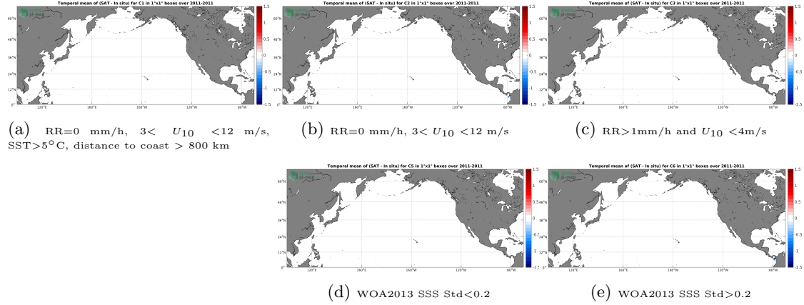
Figure 11: Temporal mean gridded over spatial boxes of size 1^\circ \times 1^\circ of \Delta SSS (Aquarius-L4-IPRC-V5-WEEKLY - Surface drifters) for 5 different subdatasets corresponding to: RR=0 mm/h, 3 < U_{10} < 12 m/s, SST > 5^\circ C , distance to coast > 800 km (a), RR=0 mm/h, 3 < U_{10} < 12 m/s (b), RR > 1 mm/h and U_{10} < 4 m/s (c), WOA2013 SSS Std < 0.2 (d), WOA2013 SSS Std > 0.2 (e).
