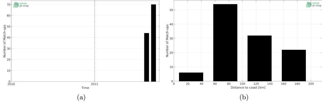
Figure 1: Number of match-ups between Surface drifters and Aquarius-L4-IPRC-V5-WEEKLY SSS as a function of time (a) and as function of the distance to coast (b) over the North Pacific Ocean Pi-MEP region and for the full satellite product period.
