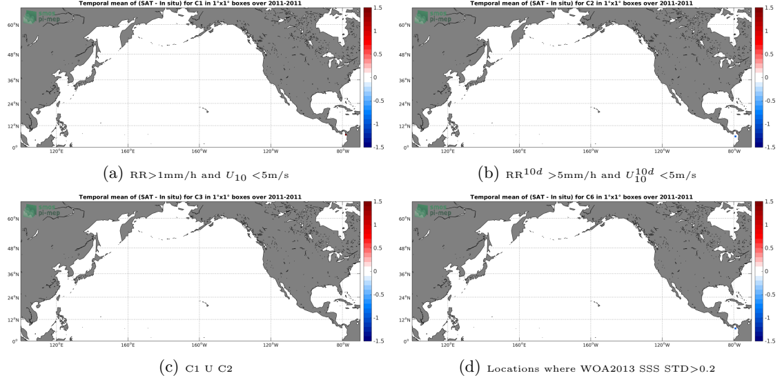
Figure 11: Temporal mean gridded over spatial boxes of size 1^\circ \times 1^\circ of \Delta SSS (Aquarius-L4-IPRC-V5-WEEKLY - Surface drifters) for 4 different subdatasets corresponding to: RR > 1\text{mm/h} and U_{10} < 5\text{m/s} (a), RR^{10d} > 5\text{mm/h} and U_{10}^{10d} < 5\text{m/s} (b), C1 U C2 (c), Locations where WOA2013 SSS STD > 0.2 (d).
