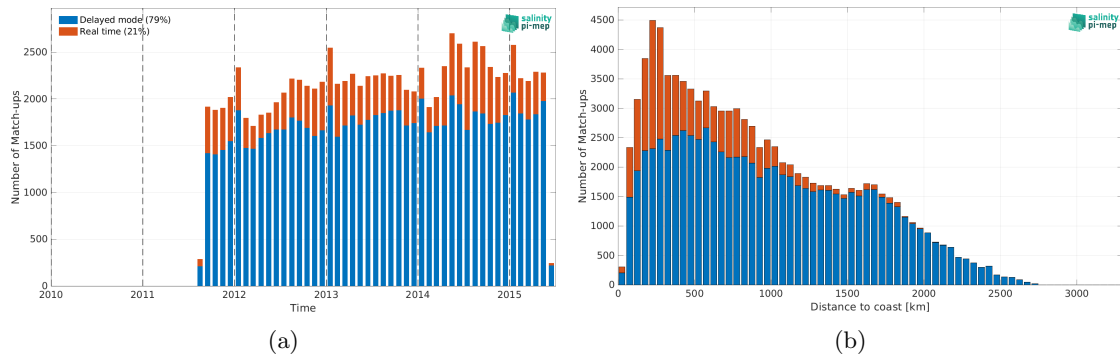
Figure 2: Number of match-ups between Argo and Aquarius SSS L4 OI v5 - Weekly (IPRC) SSS as a function of time (a) and as function of the distance to coast (b) over the North Pacific Ocean Pi-MEP region and for the full satellite product period.
