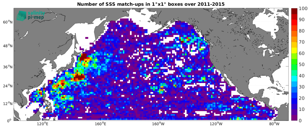
Figure 5: Number of SSS match-ups between Argo SSS and the Aquarius SSS L4 OI v5 - Weekly (IPRC) SSS product for the North Pacific Ocean Pi-MEP region over 1^\circ \times 1^\circ boxes and for the full satellite product period.
