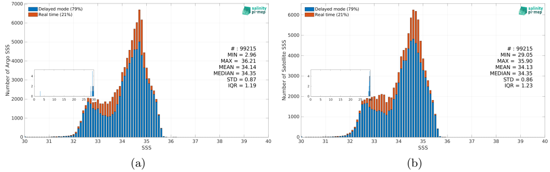
Figure 3: Histograms of SSS from Argo (a) and Aquarius SSS L4 OI v5 - Weekly (IPRC) (b) considering all match-up pairs per bins of 0.1 over the North Pacific Ocean Pi-MEP region and for the full satellite product period.
