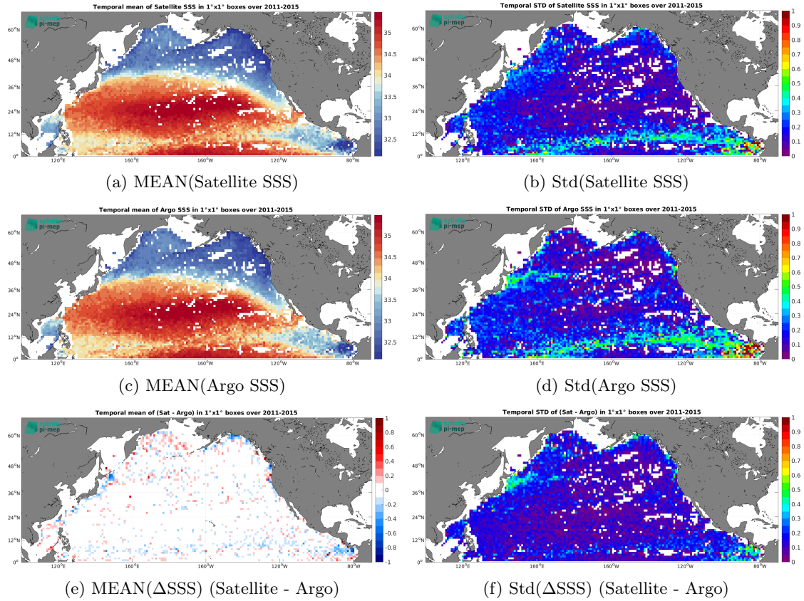
Figure 7: Temporal mean (left) and Std (right) of SSS from Aquarius SSS L4 OI v5 - Weekly (IPRC) (top), Argo (middle), and of \Delta SSS (Satellite - Argo). Only match-up pairs are used to generate these maps.
