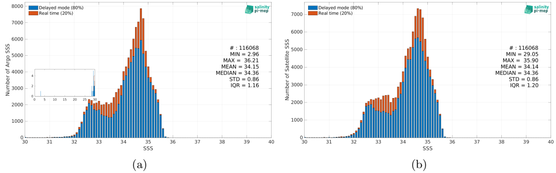
Figure 2: Histograms of SSS from Argo (a) and Aquarius SSS L4 OI v5 - Weekly (IPRC) (b) considering all match-up pairs per bins of 0.1 over the North Pacific Ocean Pi-MEP region and for the full satellite product period.
