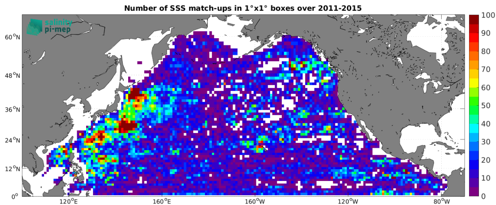
Figure 4: Number of SSS match-ups between Argo SSS and the Aquarius SSS L4 OI v5 - Weekly (IPRC) SSS product for the North Pacific Ocean Pi-MEP region over 1^\circ \times 1^\circ boxes and for the full satellite product period.
