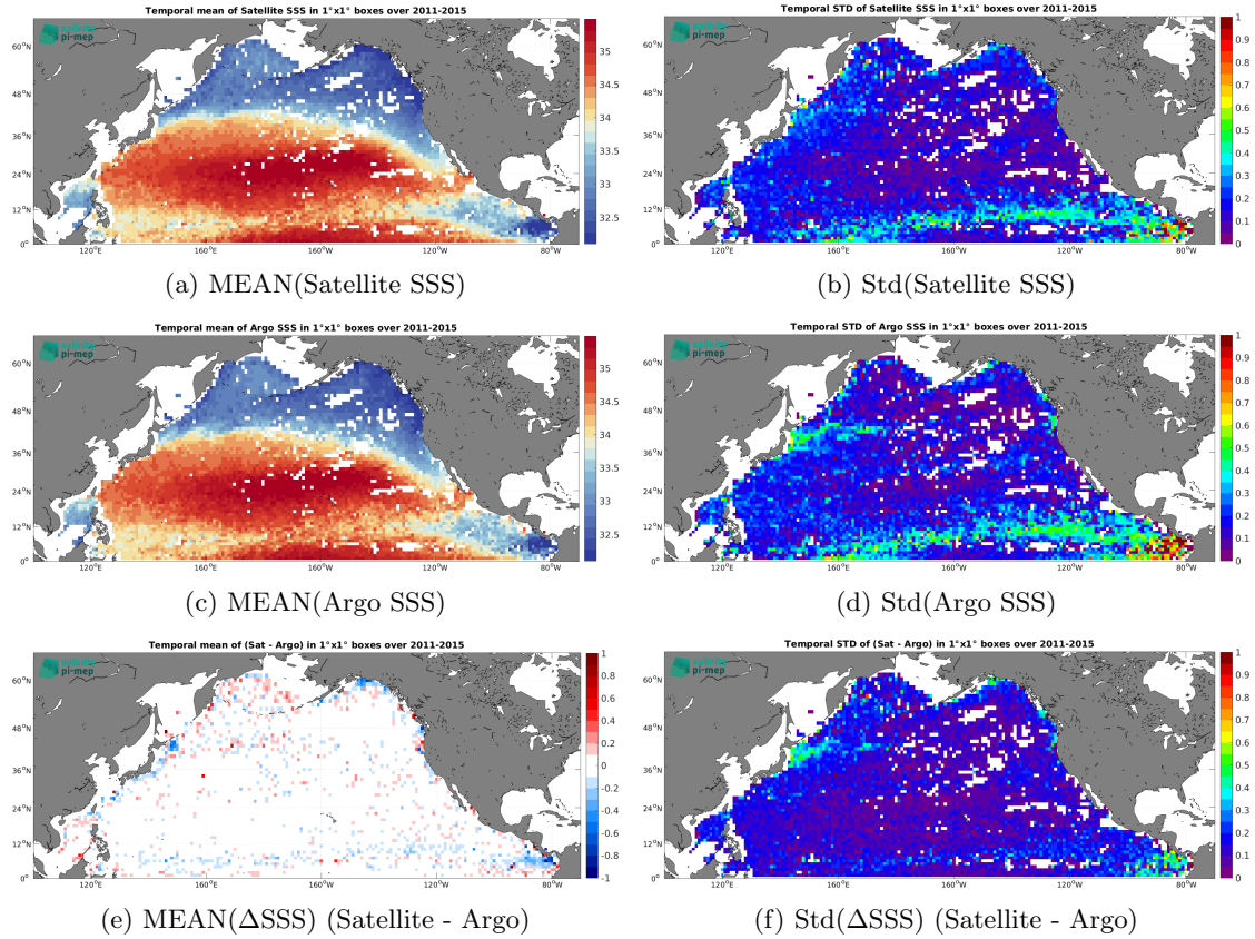
Figure 6: Temporal mean (left) and Std (right) of SSS from Aquarius SSS L4 OI v5 - Weekly (IPRC) (top), Argo (middle), and of \Delta SSS (Satellite - Argo). Only match-up pairs are used to generate these maps.
