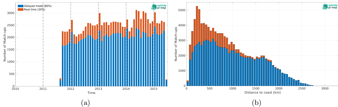
Figure 1: Number of match-ups between Argo and Aquarius SSS L4 OI v5 - Weekly (IPRC) SSS as a function of time (a) and as function of the distance to coast (b) over the North Pacific Ocean Pi-MEP region and for the full satellite product period.
