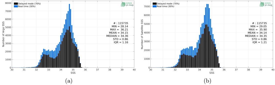
Figure 2: Histograms of SSS from Argo (a) and Aquarius-L4-IPRC-V5-WEEKLY (b) considering all match-up pairs per bins of 0.1 over the North Pacific Ocean Pi-MEP region and for the full satellite product period.
