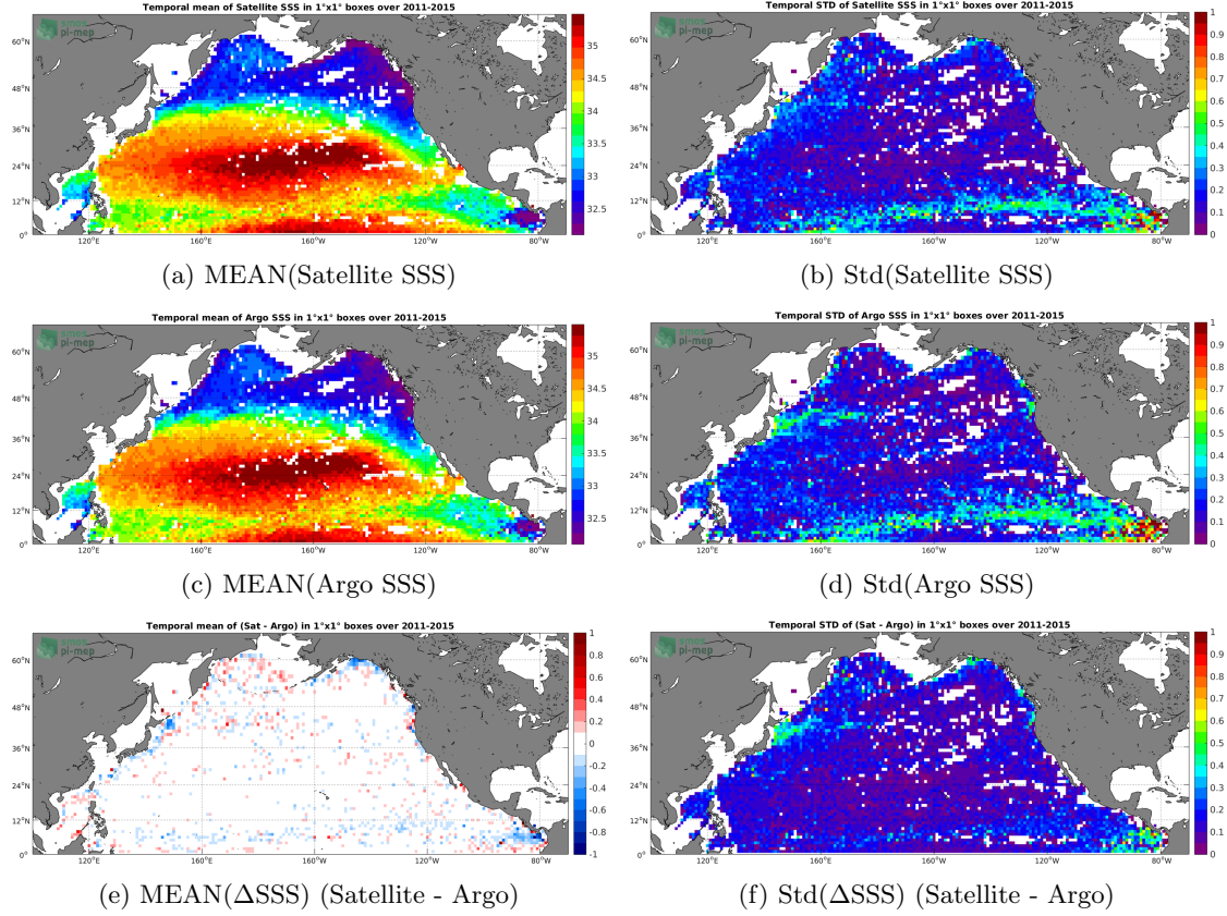
Figure 6: Temporal mean (left) and Std (right) of SSS from Aquarius-L4-IPRC-V5-WEEKLY (top), Argo (middle), and of \Delta SSS (Satellite - Argo). Only match-up pairs are used to generate these maps.
