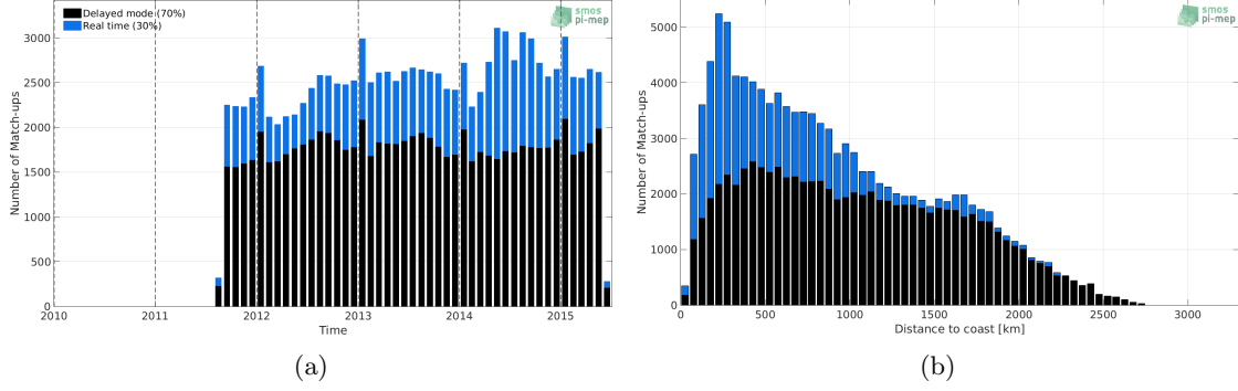
Figure 1: Number of match-ups between Argo and Aquarius-L4-IPRC-V5-WEEKLY SSS as a function of time (a) and as function of the distance to coast (b) over the North Pacific Ocean Pi-MEP region and for the full satellite product period.
