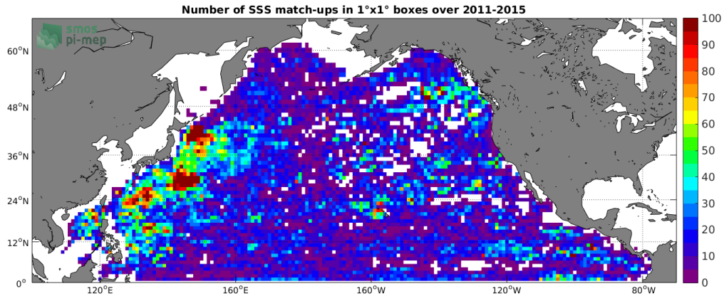
Figure 4: Number of SSS match-ups between Argo SSS and the Aquarius-L4-IPRC-V5-WEEKLY SSS product for the North Pacific Ocean Pi-MEP region over 1^\circ \times 1^\circ boxes and for the full satellite product period.
