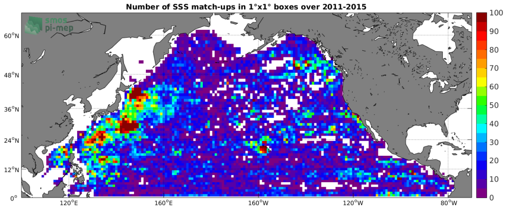
Figure 4: Number of SSS match-ups between Argo SSS and the Aquarius-L4-IPRC-V5-WEEKLY SSS product for the North Pacific Ocean Pi-MEP region over 1°x1° boxes and for the full satellite product period.
