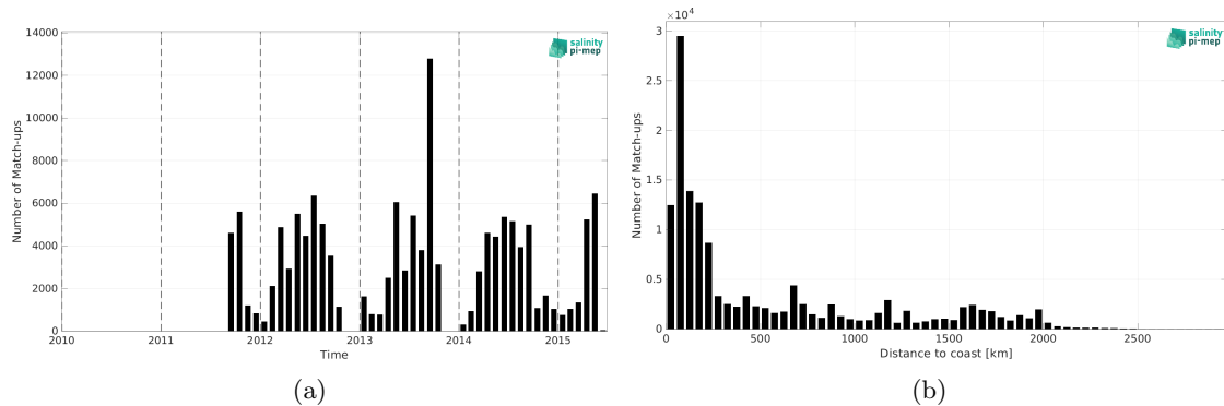
Figure 2: Number of match-ups between TSG (SAMOS) and Aquarius SSS L4 OI v5 - Monthly (IPRC) SSS as a function of time (a) and as function of the distance to coast (b) over the North Pacific Ocean Pi-MEP region and for the full satellite product period.
