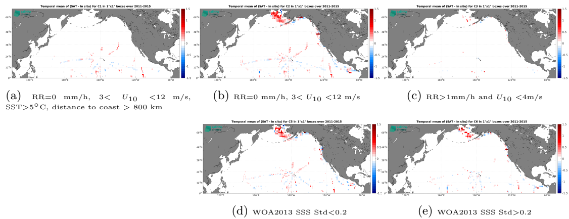
Figure 14: Temporal mean gridded over spatial boxes of size 1^\circ \times 1^\circ of \Delta\text{SSS} (Aquarius SSS L4 OI v5 - Monthly (IPRC) - TSG (SAMOS)) for 5 different subdatasets corresponding to: RR=0 mm/h, 3 < U_{10} < 12 m/s, SST > 5°C, distance to coast > 800 km (a), RR=0 mm/h, 3 < U_{10} < 12 m/s (b), RR > 1mm/h and U_{10} < 4 m/s (c), WOA2013 SSS Std < 0.2 (d), WOA2013 SSS Std > 0.2 (e).
