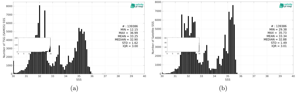
Figure 3: Histograms of SSS from TSG (SAMOS) (a) and Aquarius SSS L4 OI v5 - Monthly (IPRC) (b) considering all match-up pairs per bins of 0.1 over the North Pacific Ocean Pi-MEP region and for the full satellite product period.
