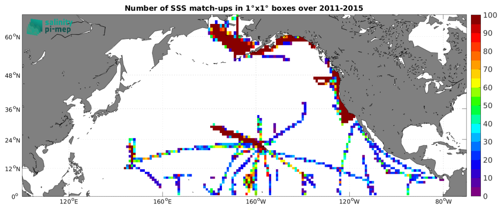
Figure 5: Number of SSS match-ups between TSG (SAMOS) SSS and the Aquarius SSS L4 OI v5 - Monthly (IPRC) SSS product for the North Pacific Ocean Pi-MEP region over 1^\circ \times 1^\circ boxes and for the full satellite product period.
