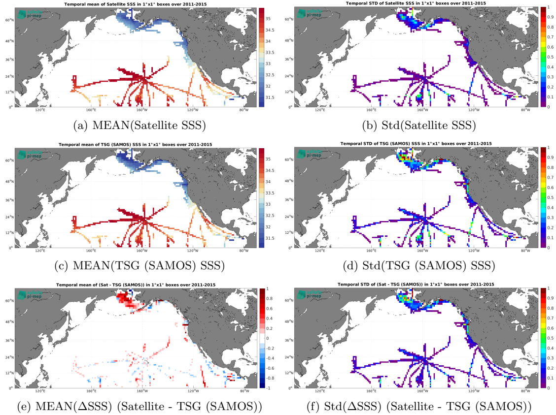
Figure 7: Temporal mean (left) and Std (right) of SSS from Aquarius SSS L4 OI v5 - Monthly (IPRC) (top), TSG (SAMOS) (middle), and of \Delta\text{SSS} (Satellite - TSG (SAMOS)). Only match-up pairs are used to generate these maps.
