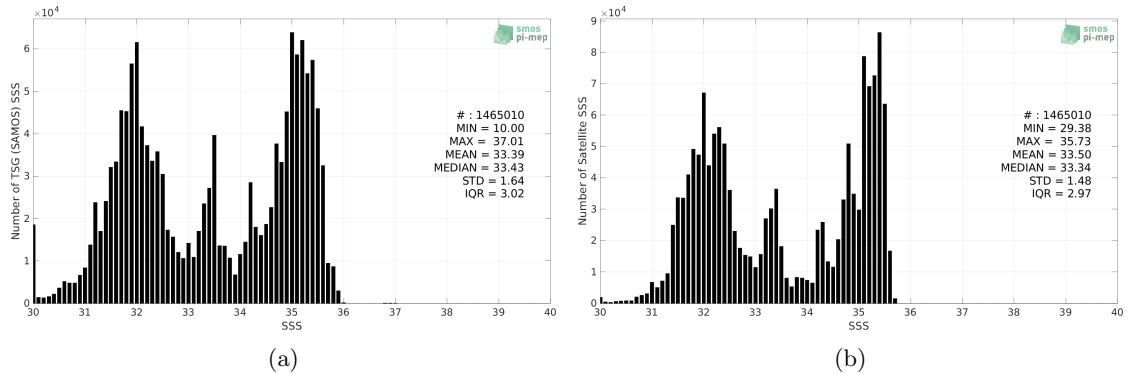
Figure 2: Histograms of SSS from TSG (SAMOS) (a) and Aquarius SSS L4 OI v5 - Monthly (IPRC) (b) considering all match-up pairs per bins of 0.1 over the North Pacific Ocean Pi-MEP region and for the full satellite product period.
