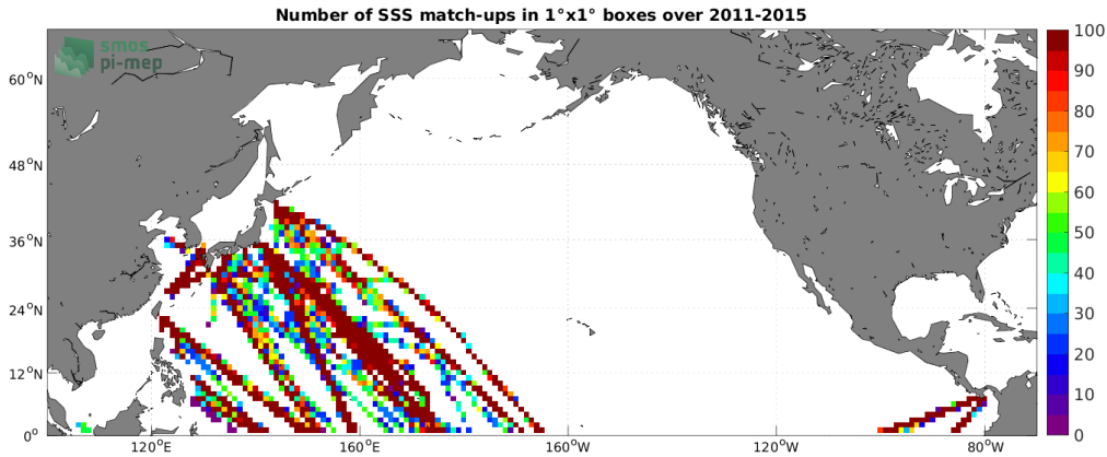
Figure 4: Number of SSS match-ups between TSG (LEGOS-DM) SSS and the Aquarius SSS L4 OI v5 - Monthly (IPRC) SSS product for the North Pacific Ocean Pi-MEP region over 1^\circ \times 1^\circ boxes and for the full satellite product period.
