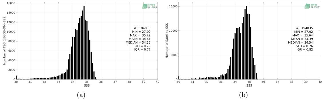
Figure 2: Histograms of SSS from TSG (LEGOS-DM) (a) and Aquarius SSS L4 OI v5 - Monthly (IPRC) (b) considering all match-up pairs per bins of 0.1 over the North Pacific Ocean Pi-MEP region and for the full satellite product period.
