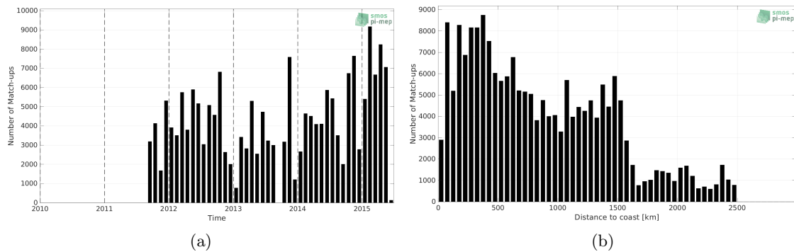
Figure 1: Number of match-ups between TSG (LEGOS-DM) and Aquarius SSS L4 OI v5 - Monthly (IPRC) SSS as a function of time (a) and as function of the distance to coast (b) over the North Pacific Ocean Pi-MEP region and for the full satellite product period.
