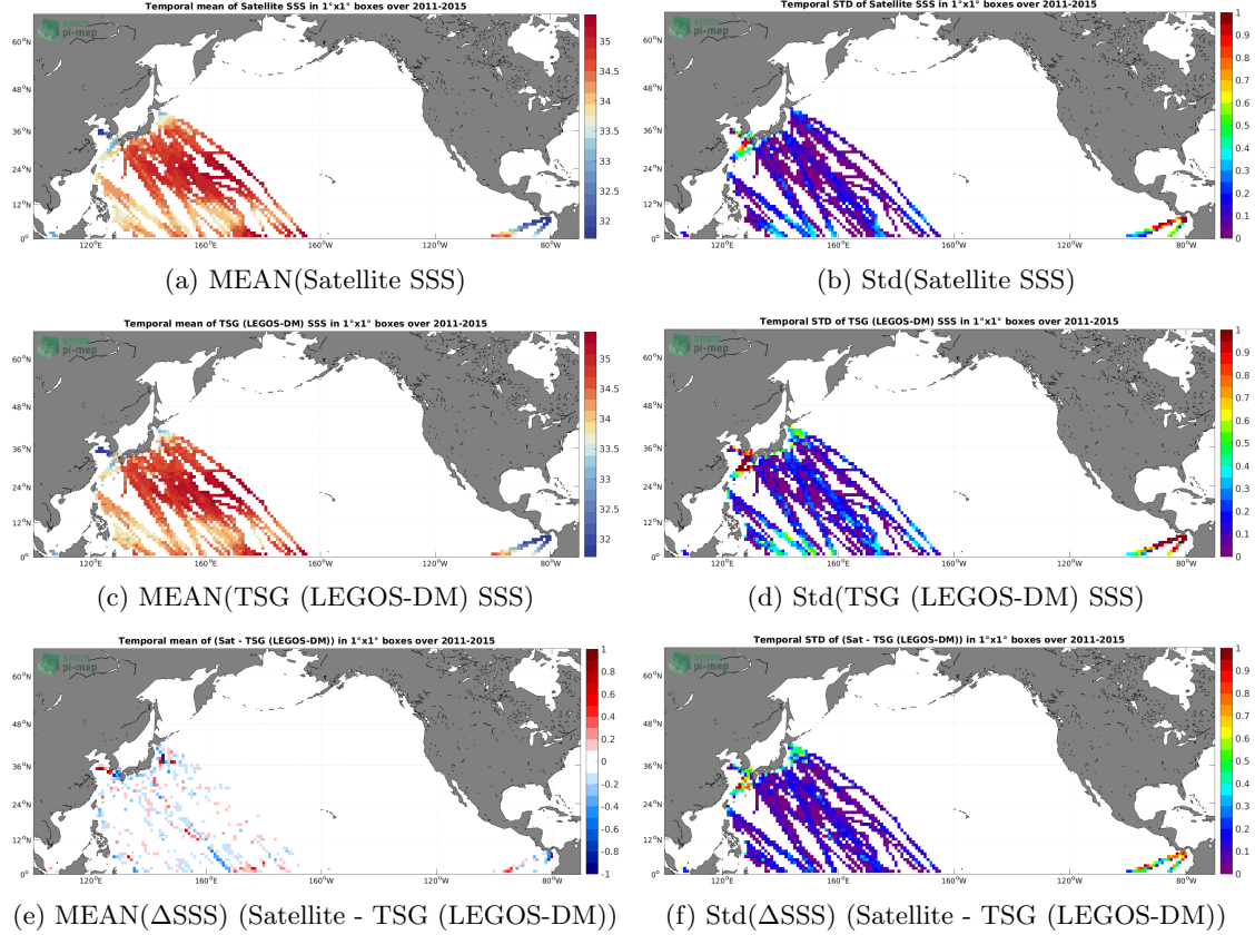
Figure 6: Temporal mean (left) and Std (right) of SSS from Aquarius SSS L4 OI v5 - Monthly (IPRC) (top), TSG (LEGOS-DM) (middle), and of \Delta\text{SSS} (Satellite - TSG (LEGOS-DM)). Only match-up pairs are used to generate these maps.
