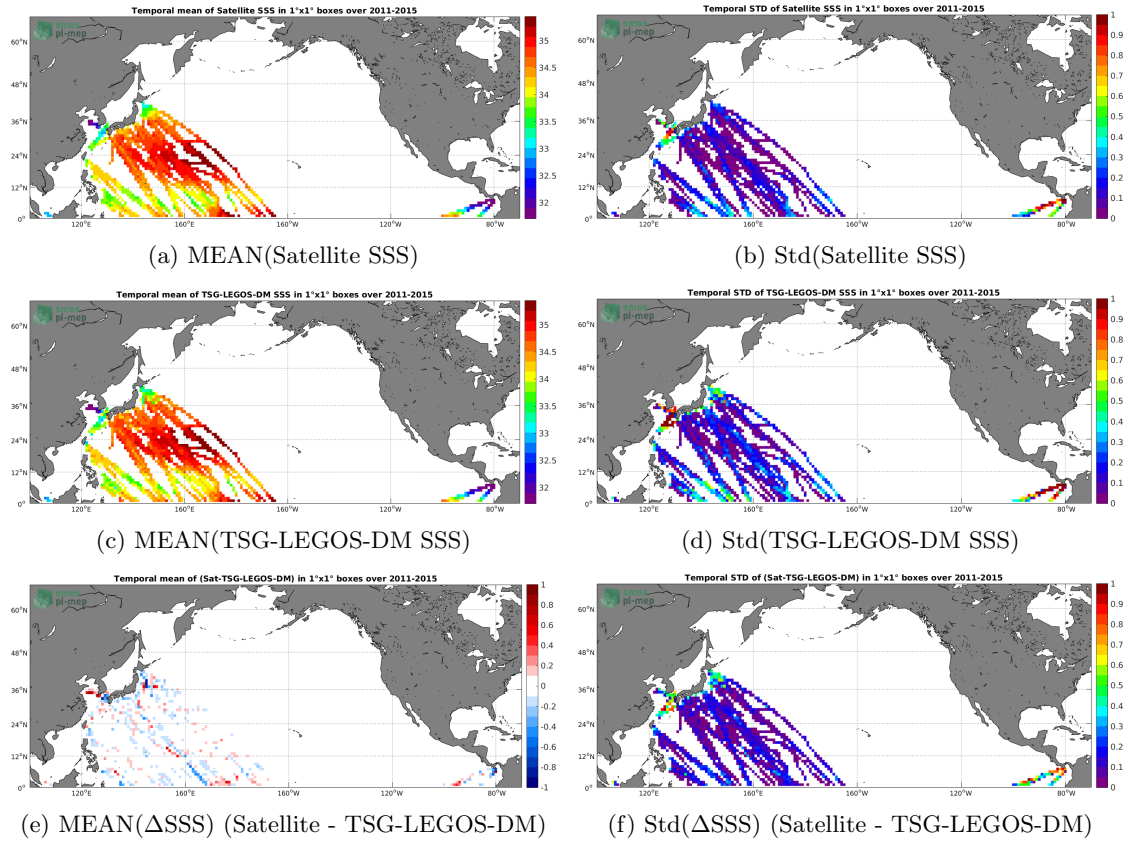
Figure 6: Temporal mean (left) and Std (right) of SSS from Aquarius-L4-IPRC-V5-MONTHLY (top), TSG-LEGOS-DM (middle), and of \Delta SSS (Satellite - TSG-LEGOS-DM). Only match-up pairs are used to generate these maps.
