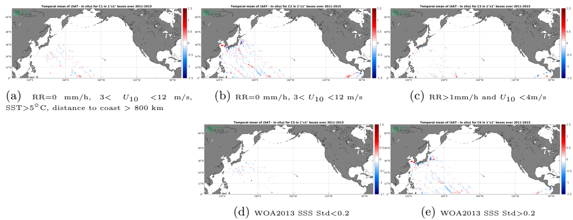
Figure 12: Temporal mean gridded over spatial boxes of size 1^\circ \times 1^\circ of \Delta SSS (Aquarius-L4-IPRC-V5-MONTHLY - TSG-LEGOS-DM) for 5 different subdatasets corresponding to:RR=0 mm/h, 3 < U_{10} < 12 m/s, SST >5^\circ C, distance to coast > 800 km (a), RR=0 mm/h, 3 < U_{10} < 12 m/s (b), RR >1 mm/h and U_{10} < 4 m/s (c), WOA2013 SSS Std <0.2 (d), WOA2013 SSS Std >0.2 (e).
