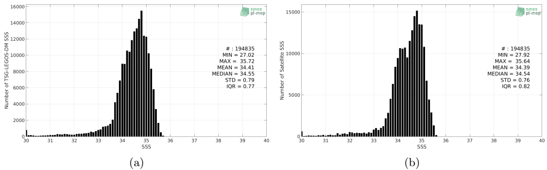
Figure 2: Histograms of SSS from TSG-LEGOS-DM (a) and Aquarius-L4-IPRC-V5-MONTHLY (b) considering all match-up pairs per bins of 0.1 over the North Pacific Ocean Pi-MEP region and for the full satellite product period.
