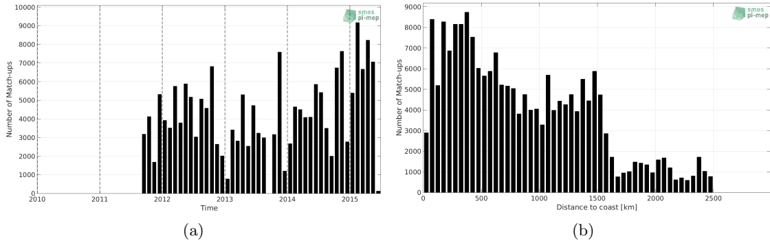
Figure 1: Number of match-ups between TSG-LEGOS-DM and Aquarius-L4-IPRC-V5-MONTHLY SSS as a function of time (a) and as function of the distance to coast (b) over the North Pacific Ocean Pi-MEP region and for the full satellite product period.
