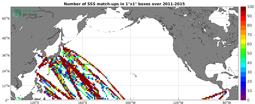
Figure 4: Number of SSS match-ups between TSG-LEGOS-DM SSS and the Aquarius-L4-IPRC-V5-MONTHLY SSS product for the North Pacific Ocean Pi-MEP region over 1^\circ \times 1^\circ boxes and for the full satellite product period.
