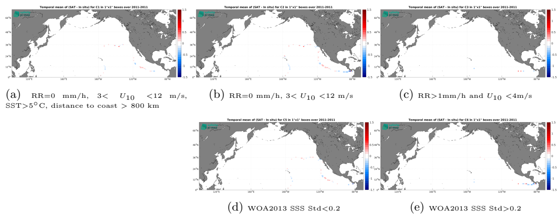
Figure 14: Temporal mean gridded over spatial boxes of size 1^\circ \times 1^\circ of \Delta\text{SSS} (Aquarius SSS L4 OI v5 - Monthly (IPRC) - TSG (GOSUD-Sailing-ship)) for 5 different subdatasets corresponding to:RR=0 mm/h, 3 < U_{10} < 12 m/s, SST>5°C, distance to coast > 800 km (a), RR=0 mm/h, 3 < U_{10} < 12 m/s (b), RR>1mm/h and U_{10} < 4 m/s (c), WOA2013 SSS Std<0.2 (d), WOA2013 SSS Std>0.2 (e).
