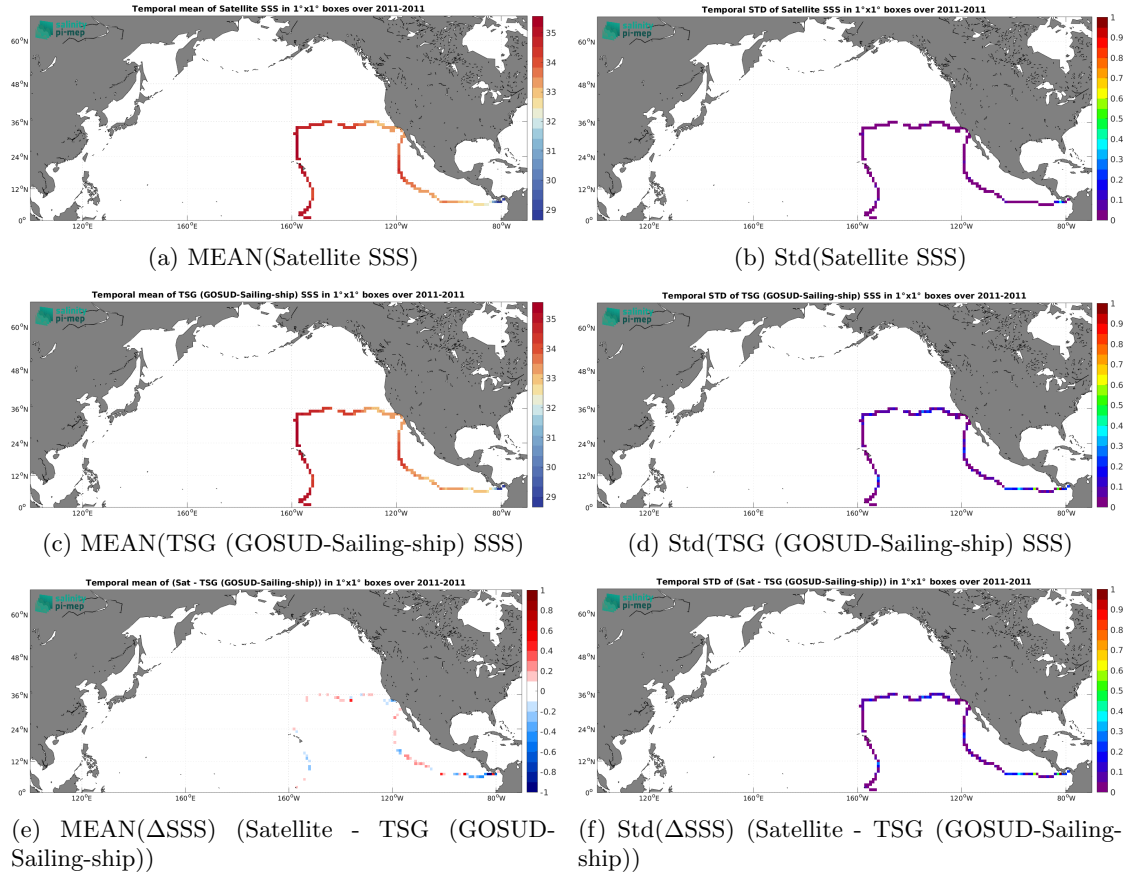
Figure 7: Temporal mean (left) and Std (right) of SSS from Aquarius SSS L4 OI v5 - Monthly (IPRC) (top), TSG (GOSUD-Sailing-ship) (middle), and of \Delta\text{SSS} (Satellite - TSG (GOSUD-Sailing-ship)). Only match-up pairs are used to generate these maps.
