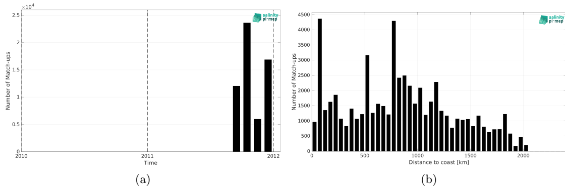
Figure 2: Number of match-ups between TSG (GOSUD-Sailing-ship) and Aquarius SSS L4 OI v5 - Monthly (IPRC) SSS as a function of time (a) and as function of the distance to coast (b) over the North Pacific Ocean Pi-MEP region and for the full satellite product period.
