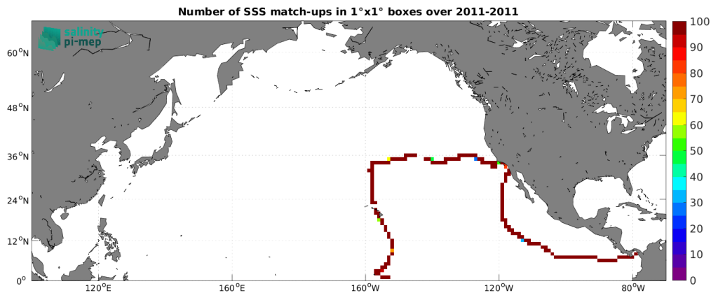
Figure 5: Number of SSS match-ups between TSG (GOSUD-Sailing-ship) SSS and the Aquarius SSS L4 OI v5 - Monthly (IPRC) SSS product for the North Pacific Ocean Pi-MEP region over 1^\circ \times 1^\circ boxes and for the full satellite product period.
