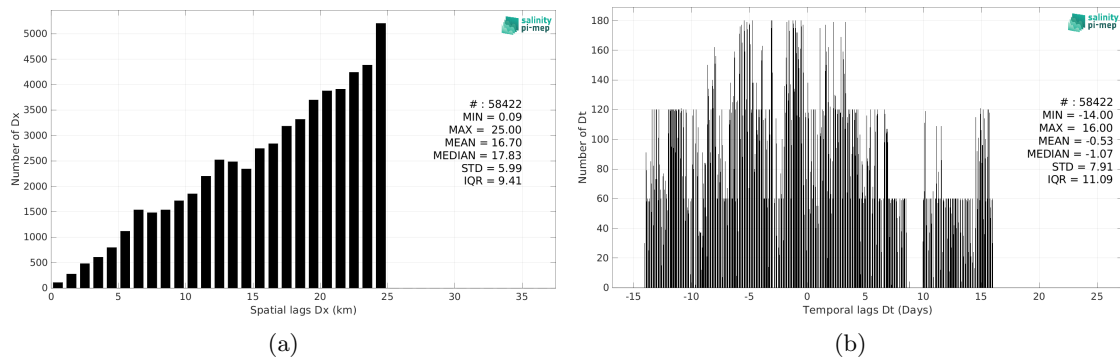
Figure 6: Histograms of the spatial (a) and temporal (b) lags between the location/time of the TSG (GOSUD-Sailing-ship) measurement and the date of the corresponding Aquarius SSS L4 OI v5 - Monthly (IPRC) SSS pixel.
