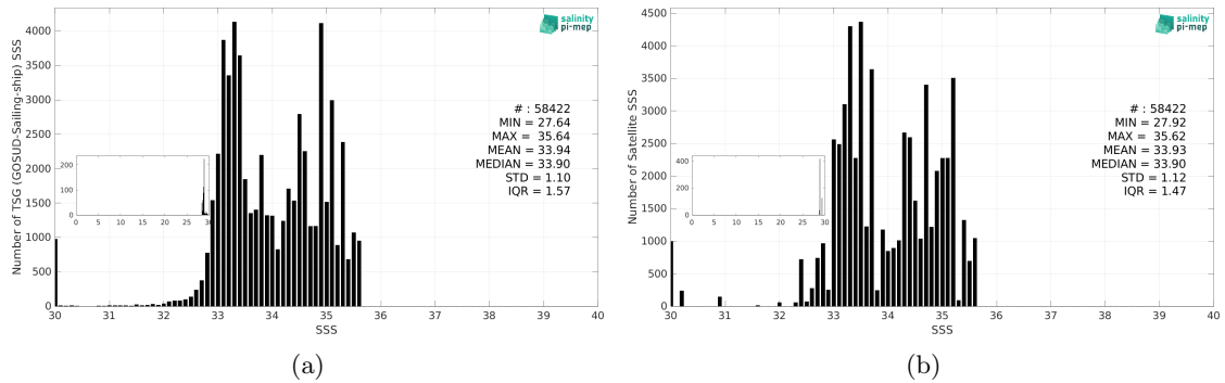
Figure 3: Histograms of SSS from TSG (GOSUD-Sailing-ship) (a) and Aquarius SSS L4 OI v5 - Monthly (IPRC) (b) considering all match-up pairs per bins of 0.1 over the North Pacific Ocean Pi-MEP region and for the full satellite product period.
