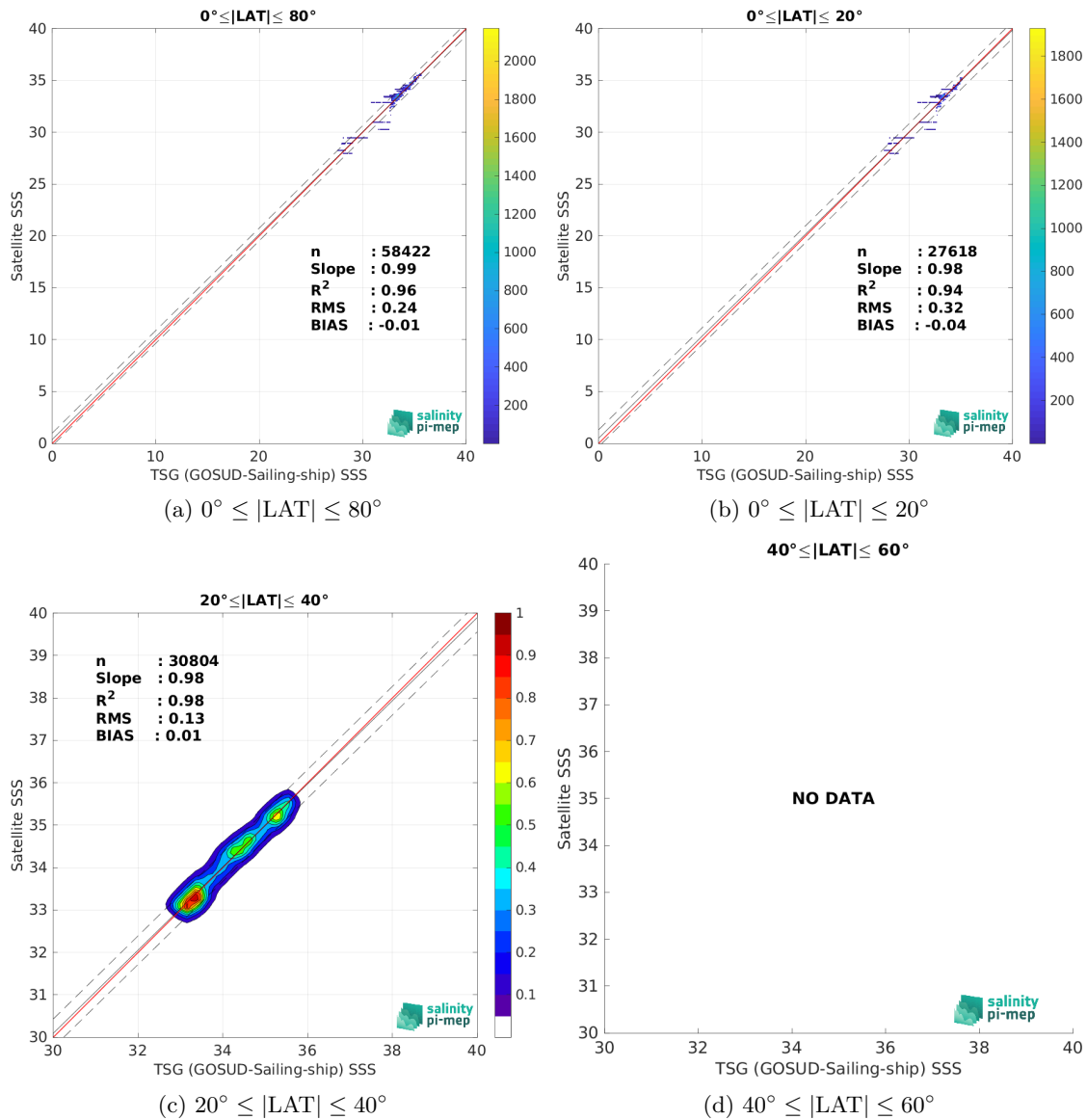
Figure 10: Contour maps of the concentration of Aquarius SSS L4 OI v5 - Monthly (IPRC) SSS (y-axis) versus TSG (GOSUD-Sailing-ship) SSS (x-axis) at match-up pairs for different latitude bands. For each plot, the red line shows x=y . The black thin and dashed lines indicate a linear fit through the data cloud and the \pm 95\% confidence levels, respectively. The number match-up pairs n , the slope and R^2 coefficient of the linear fit, the root mean square (RMS) and the mean bias between satellite and in situ data are indicated for each latitude band in each plots.
