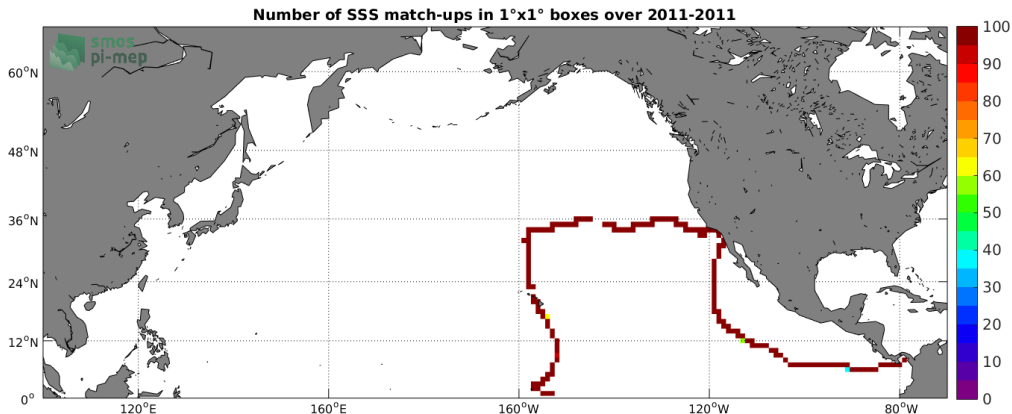
Figure 4: Number of SSS match-ups between TSG (GOSUD-Sailing-ship) SSS and the Aquarius SSS L4 OI v5 - Monthly (IPRC) SSS product for the North Pacific Ocean Pi-MEP region over 1^\circ \times 1^\circ boxes and for the full satellite product period.
