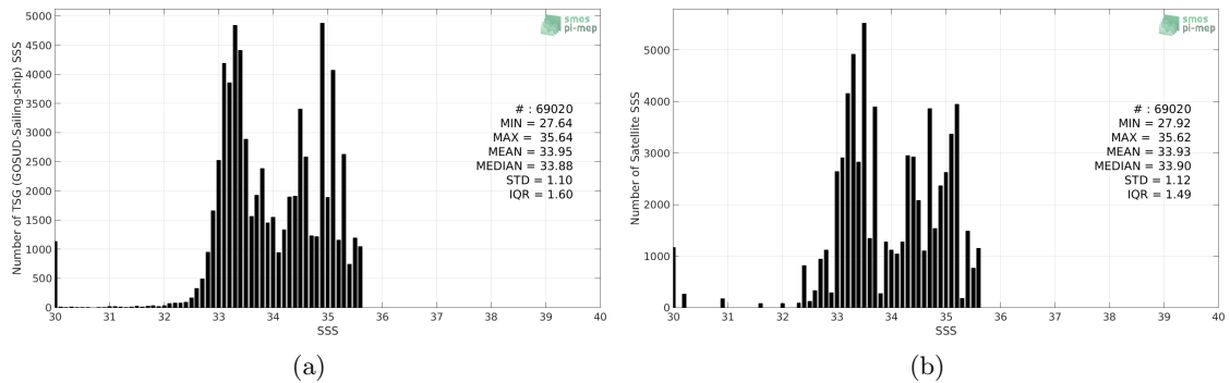
Figure 2: Histograms of SSS from TSG (GOSUD-Sailing-ship) (a) and Aquarius SSS L4 OI v5 - Monthly (IPRC) (b) considering all match-up pairs per bins of 0.1 over the North Pacific Ocean Pi-MEP region and for the full satellite product period.
