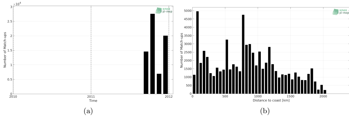
Figure 1: Number of match-ups between TSG (GOSUD-Sailing-ship) and Aquarius SSS L4 OI v5 - Monthly (IPRC) SSS as a function of time (a) and as function of the distance to coast (b) over the North Pacific Ocean Pi-MEP region and for the full satellite product period.
