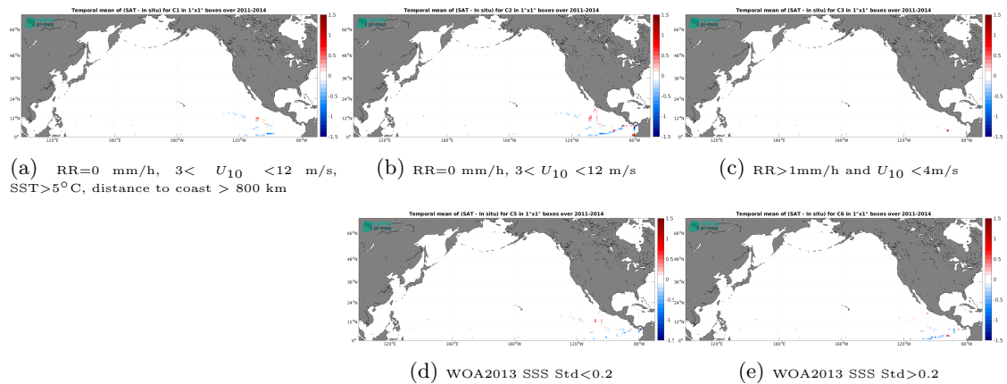
Figure 12: Temporal mean gridded over spatial boxes of size 1^{\circ}\times 1^{\circ} of \Delta SSS (Aquarius SSS L4 OI v5 - Monthly (IPRC) - TSG (GOSUD-Research-vessel)) for 5 different subdatasets corresponding to:RR=0 mm/h, 3 < U_{10} < 12 m/s, SST >5^{\circ}\text{C} , distance to coast > 800 km (a), RR=0 mm/h, 3 < U_{10} < 12 m/s (b), RR >1 mm/h and U_{10} < 4 m/s (c), WOA2013 SSS Std <0.2 (d), WOA2013 SSS Std >0.2 (e).
