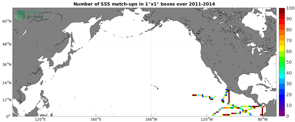
Figure 4: Number of SSS match-ups between TSG (GOSUD-Research-vessel) SSS and the Aquarius SSS L4 OI v5 - Monthly (IPRC) SSS product for the North Pacific Ocean Pi-MEP region over 1^\circ \times 1^\circ boxes and for the full satellite product period.
