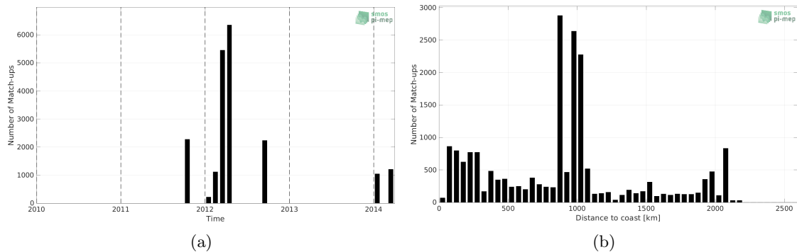
Figure 1: Number of match-ups between TSG (GOSUD-Research-vessel) and Aquarius SSS L4 OI v5 - Monthly (IPRC) SSS as a function of time (a) and as function of the distance to coast (b) over the North Pacific Ocean Pi-MEP region and for the full satellite product period.
