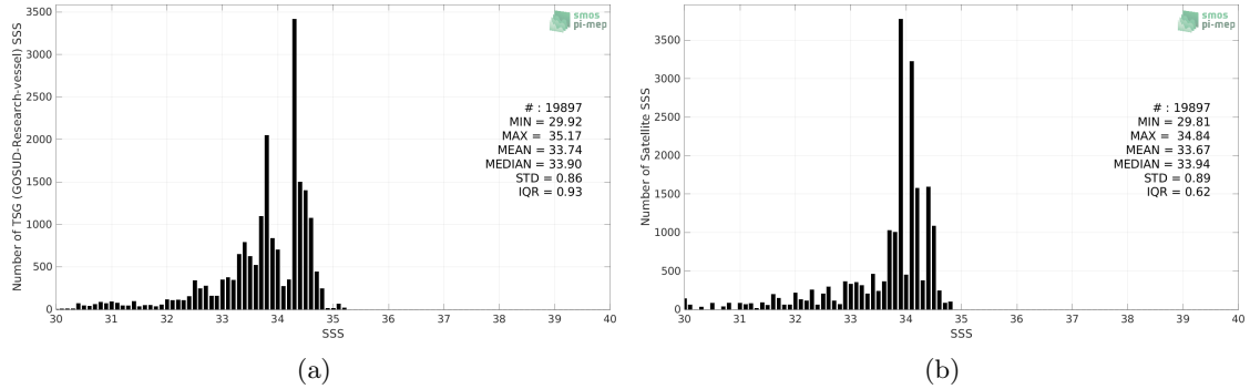
Figure 2: Histograms of SSS from TSG (GOSUD-Research-vessel) (a) and Aquarius SSS L4 OI v5 - Monthly (IPRC) (b) considering all match-up pairs per bins of 0.1 over the North Pacific Ocean Pi-MEP region and for the full satellite product period.
