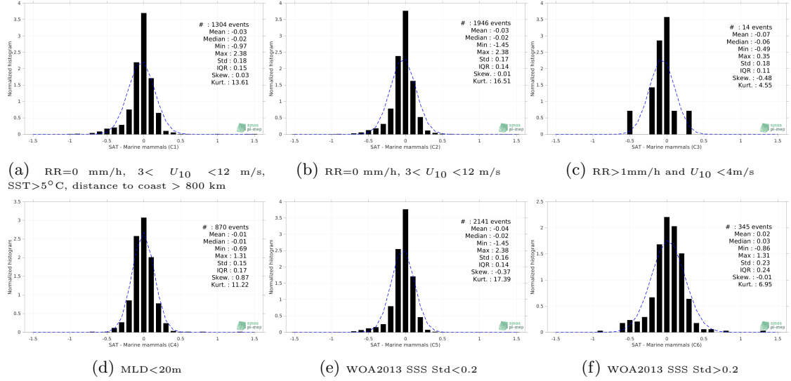
Figure 13: Normalized histogram of \Delta SSS (Aquarius SSS L4 OI v5 - Monthly (IPRC) - Marine mammals) for 6 different subdatasets corresponding to: RR=0 mm/h, 3 < U_{10} < 12 m/s, SST > 5°C, distance to coast > 800 km (a), RR=0 mm/h, 3 < U_{10} < 12 m/s (b), RR > 1mm/h and U_{10} < 4 m/s (c), MLD < 20m (d), WOA2013 SSS Std < 0.2 (e), WOA2013 SSS Std > 0.2 (f).
