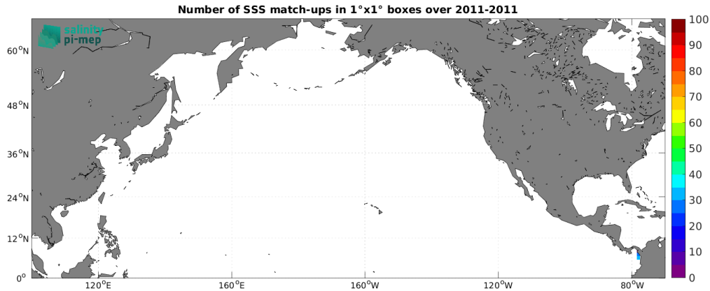
Figure 4: Number of SSS match-ups between Surface drifters SSS and the Aquarius SSS L4 OI v5 - Monthly (IPRC) SSS product for the North Pacific Ocean Pi-MEP region over 1^\circ \times 1^\circ boxes and for the full satellite product period.
