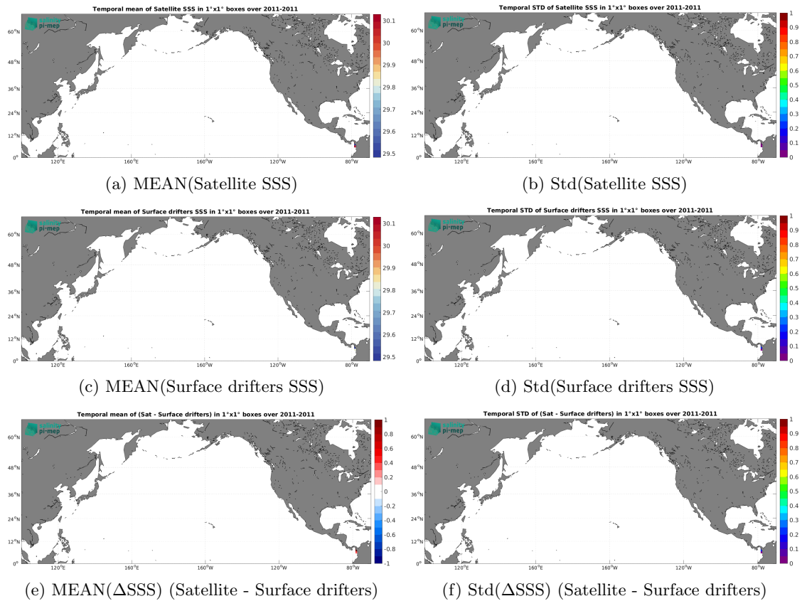
Figure 6: Temporal mean (left) and Std (right) of SSS from Aquarius SSS L4 OI v5 - Monthly (IPRC) (top), Surface drifters (middle), and of \Delta SSS (Satellite - Surface drifters). Only match-up pairs are used to generate these maps.
