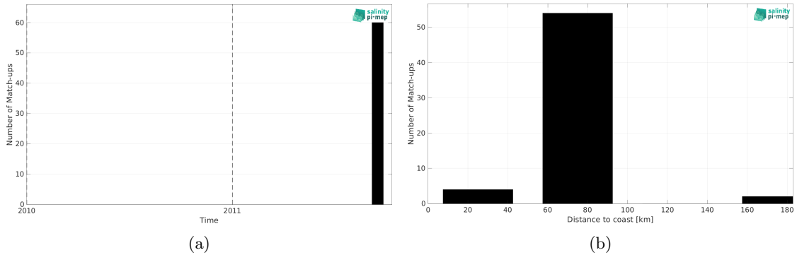
Figure 2: Number of match-ups between Surface drifters and Aquarius SSS L4 OI v5 - Monthly (IPRC) SSS as a function of time (a) and as function of the distance to coast (b) over the North Pacific Ocean Pi-MEP region and for the full satellite product period.
