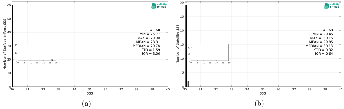
Figure 3: Histograms of SSS from Surface drifters (a) and Aquarius SSS L4 OI v5 - Monthly (IPRC) (b) considering all match-up pairs per bins of 0.1 over the North Pacific Ocean Pi-MEP region and for the full satellite product period.
