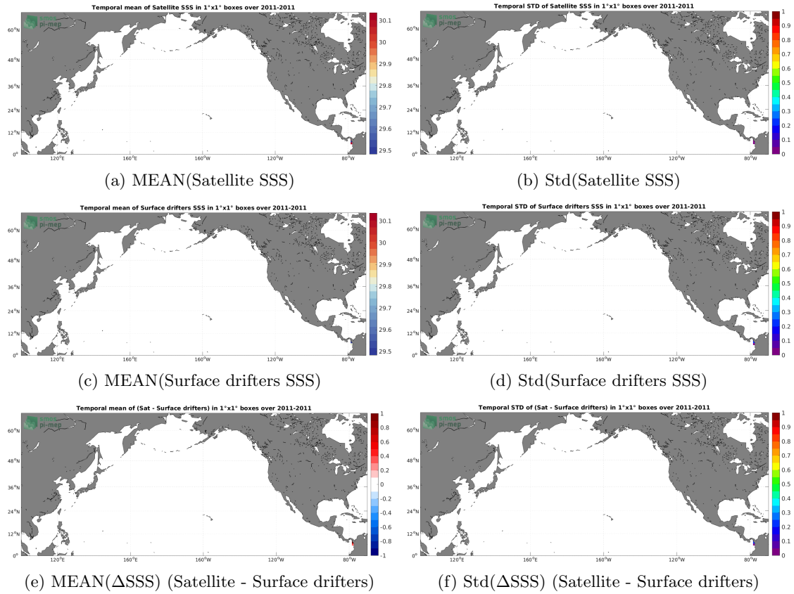
Figure 5: Temporal mean (left) and Std (right) of SSS from Aquarius SSS L4 OI v5 - Monthly (IPRC) (top), Surface drifters (middle), and of \Delta SSS (Satellite - Surface drifters). Only match-up pairs are used to generate these maps.
