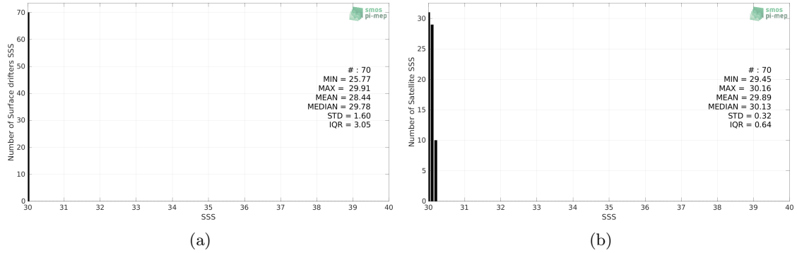
Figure 2: Histograms of SSS from Surface drifters (a) and Aquarius SSS L4 OI v5 - Monthly (IPRC) (b) considering all match-up pairs per bins of 0.1 over the North Pacific Ocean Pi-MEP region and for the full satellite product period.
