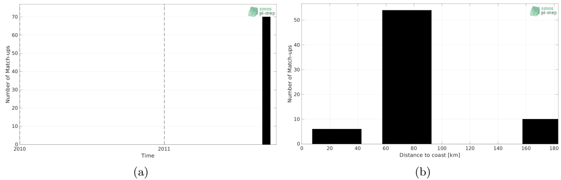
Figure 1: Number of match-ups between Surface drifters and Aquarius SSS L4 OI v5 - Monthly (IPRC) SSS as a function of time (a) and as function of the distance to coast (b) over the North Pacific Ocean Pi-MEP region and for the full satellite product period.
