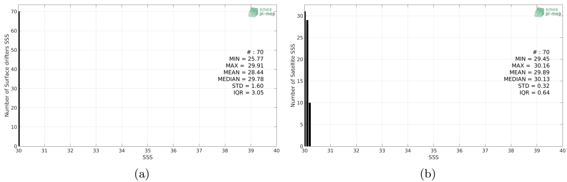
Figure 2: Histograms of SSS from Surface drifters (a) and Aquarius-L4-IPRC-V5-MONTHLY (b) considering all match-up pairs per bins of 0.1 over the North Pacific Ocean Pi-MEP region and for the full satellite product period.
