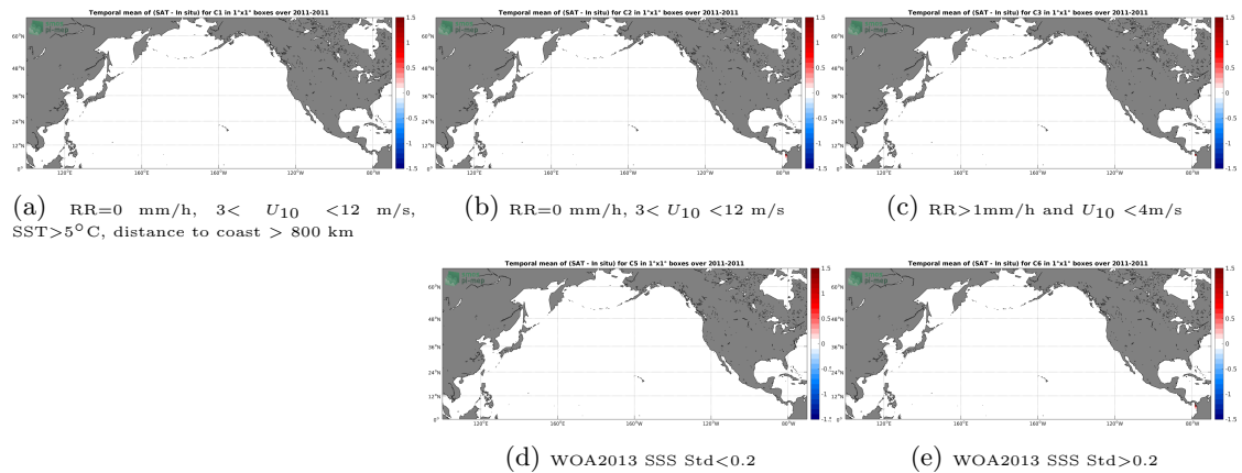
Figure 11: Temporal mean gridded over spatial boxes of size 1^\circ \times 1^\circ of \Delta SSS (Aquarius-L4-IPRC-V5-MONTHLY - Surface drifters) for 5 different subdatasets corresponding to:RR=0 mm/h, 3 < U_{10} < 12 m/s, SST >5^\circ\text{C} , distance to coast > 800 km (a), RR=0 mm/h, 3 < U_{10} < 12 m/s (b), RR >1 mm/h and U_{10} < 4 m/s (c), WOA2013 SSS Std <0.2 (d), WOA2013 SSS Std >0.2 (e).
