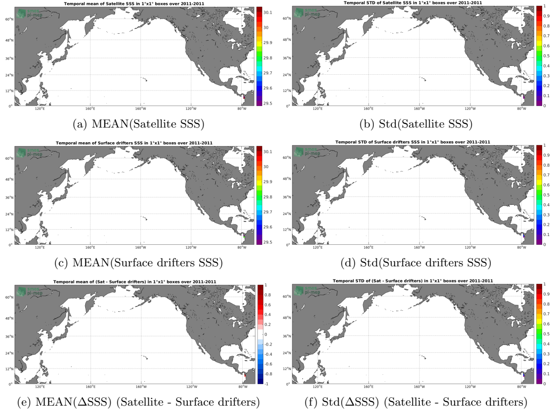
Figure 5: Temporal mean (left) and Std (right) of SSS from Aquarius-L4-IPRC-V5-MONTHLY (top), Surface drifters (middle), and of \Delta SSS (Satellite - Surface drifters). Only match-up pairs are used to generate these maps.
