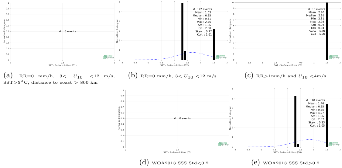
Figure 12: Normalized histogram of \Delta SSS (Aquarius-L4-IPRC-V5-MONTHLY - Surface drifters) for 5 different subdatasets corresponding to: RR=0 mm/h, 3 < U_{10} < 12 m/s, SST > 5°C, distance to coast > 800 km (a), RR=0 mm/h, 3 < U_{10} < 12 m/s (b), RR > 1mm/h and U_{10} < 4 m/s (c), WOA2013 SSS Std < 0.2 (d), WOA2013 SSS Std > 0.2 (e).
