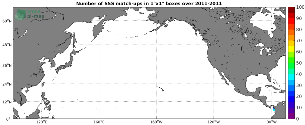
Figure 3: Number of SSS match-ups between Surface drifters SSS and the Aquarius-L4-IPRC-V5-MONTHLY SSS product for the North Pacific Ocean Pi-MEP region over 1°x1° boxes and for the full satellite product period.
