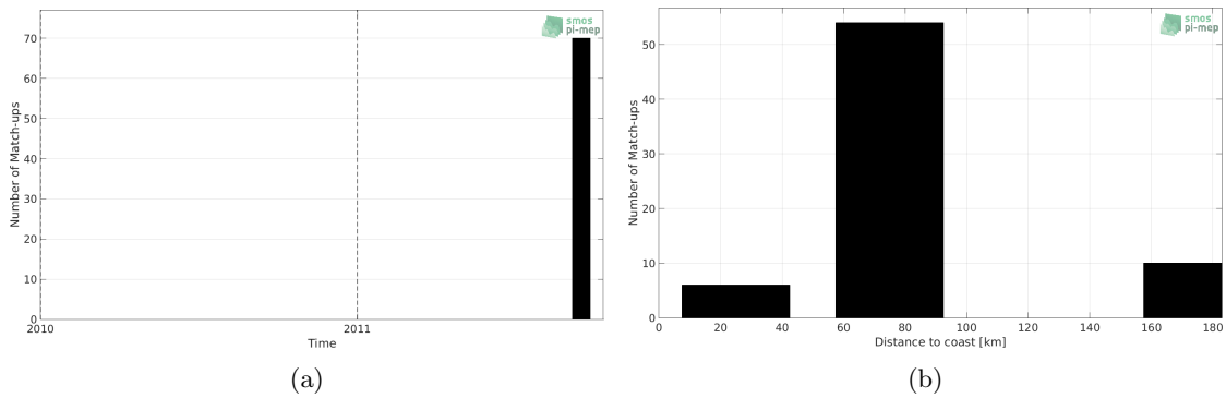
Figure 1: Number of match-ups between Surface drifters and Aquarius-L4-IPRC-V5-MONTHLY SSS as a function of time (a) and as function of the distance to coast (b) over the North Pacific Ocean Pi-MEP region and for the full satellite product period.
