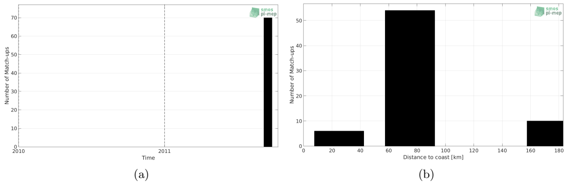
Figure 1: Number of match-ups between Surface drifters and Aquarius-L4-IPRC-V5-MONTHLY SSS as a function of time (a) and as function of the distance to coast (b) over the North Pacific Ocean Pi-MEP region and for the full satellite product period.
