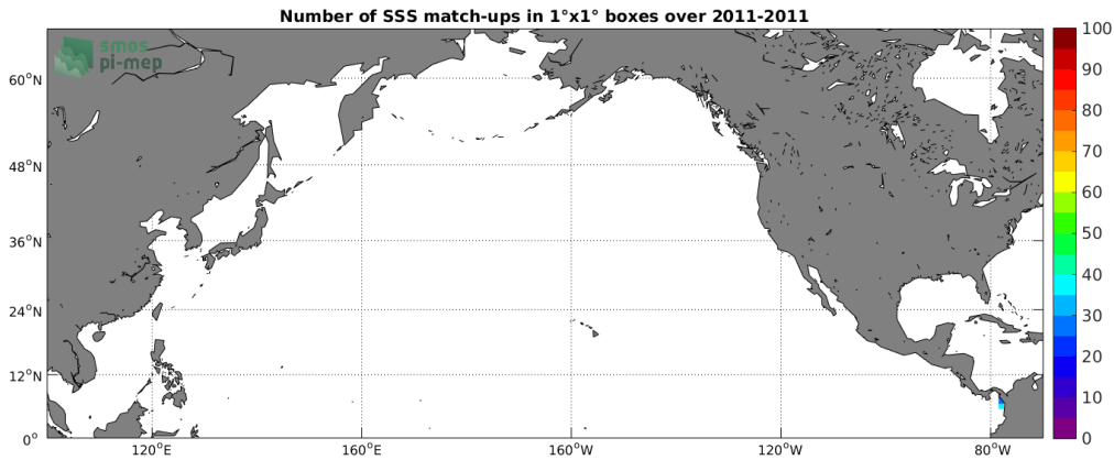
Figure 3: Number of SSS match-ups between Surface drifters SSS and the Aquarius-L4-IPRC-V5-MONTHLY SSS product for the North Pacific Ocean Pi-MEP region over 1^\circ \times 1^\circ boxes and for the full satellite product period.
