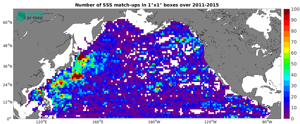
Figure 5: Number of SSS match-ups between Argo SSS and the Aquarius SSS L4 OI v5 - Monthly (IPRC) SSS product for the North Pacific Ocean Pi-MEP region over 1^\circ \times 1^\circ boxes and for the full satellite product period.
