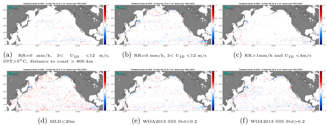
Figure 14: Temporal mean gridded over spatial boxes of size 1^\circ \times 1^\circ of \Delta SSS (Aquarius SSS L4 OI v5 - Monthly (IPRC) - Argo) for 6 different subdatasets corresponding to:RR=0 mm/h, 3 < U_{10} < 12 m/s, SST >5^\circ C, distance to coast > 800 km (a), RR=0 mm/h, 3 < U_{10} < 12 m/s (b), RR >1 mm/h and U_{10} < 4 m/s (c),MLD <20 m (d),WOA2013 SSS Std <0.2 (e),WOA2013 SSS Std >0.2 (f).
