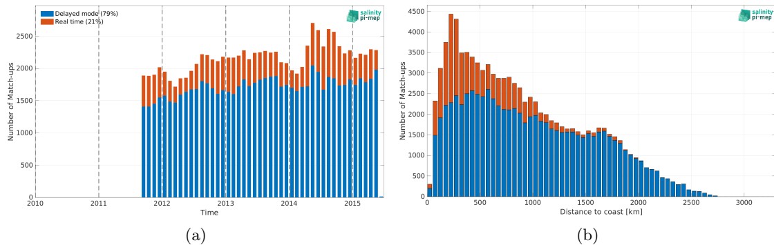
Figure 2: Number of match-ups between Argo and Aquarius SSS L4 OI v5 - Monthly (IPRC) SSS as a function of time (a) and as function of the distance to coast (b) over the North Pacific Ocean Pi-MEP region and for the full satellite product period.
