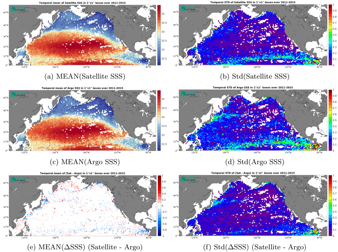
Figure 7: Temporal mean (left) and Std (right) of SSS from Aquarius SSS L4 OI v5 - Monthly (IPRC) (top), Argo (middle), and of \Delta\text{SSS} (Satellite - Argo). Only match-up pairs are used to generate these maps.
