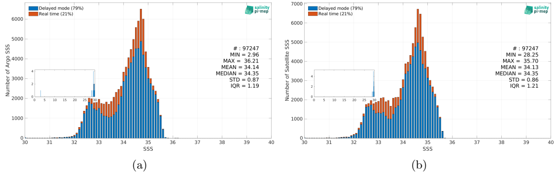
Figure 3: Histograms of SSS from Argo (a) and Aquarius SSS L4 OI v5 - Monthly (IPRC) (b) considering all match-up pairs per bins of 0.1 over the North Pacific Ocean Pi-MEP region and for the full satellite product period.
